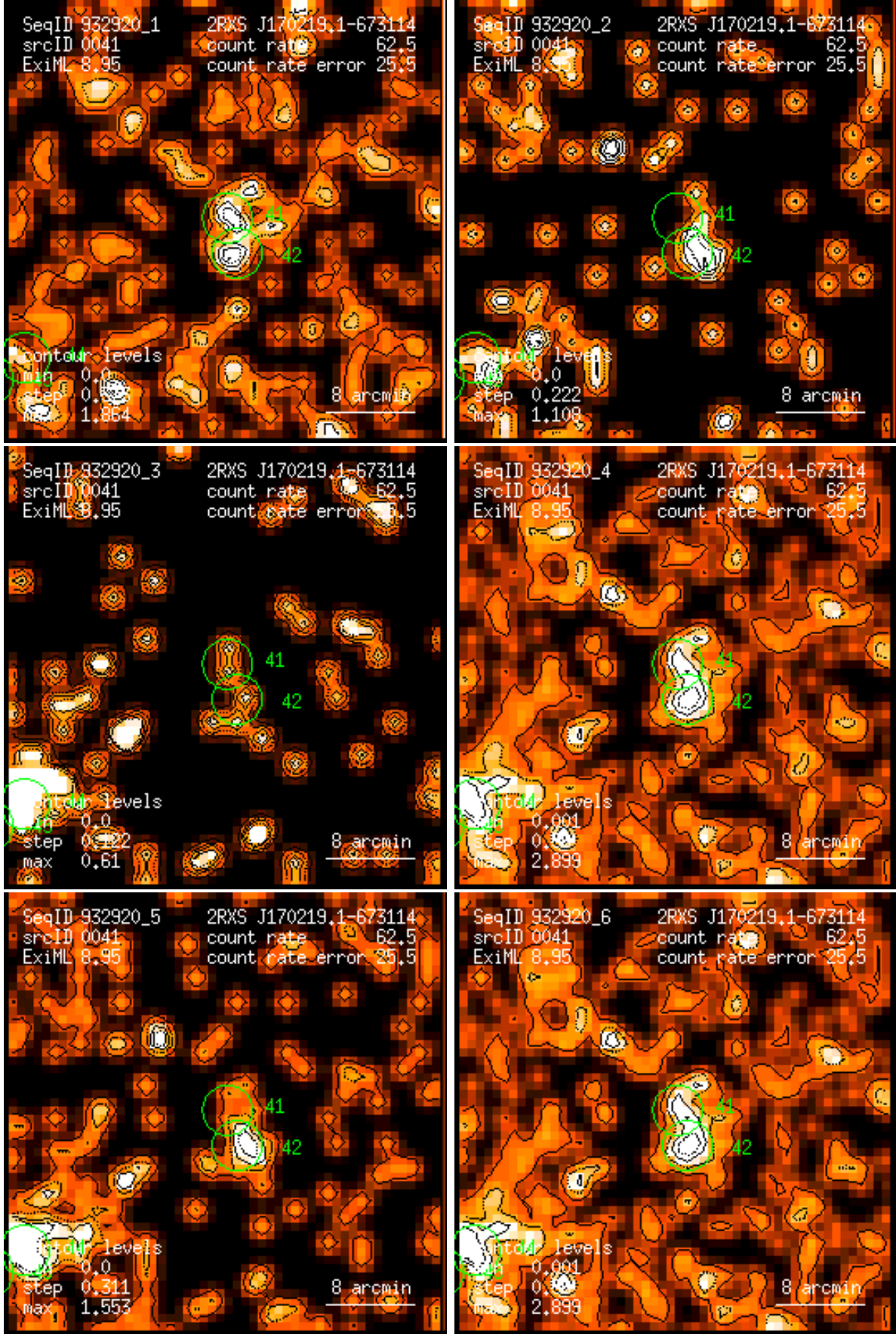
Figure 41: RASS 932920: detection 0041: band rate images, Gaussian filter: (1) PSPC channels 11 – 41, (2) 52 – 90, (3) 91 – 201, (4) 11 – 235, (5) 52 – 201, (6) 11 – 201. Broad band rates in counts/ks. Band rate contour levels in counts/ks/arcmin 2 .
