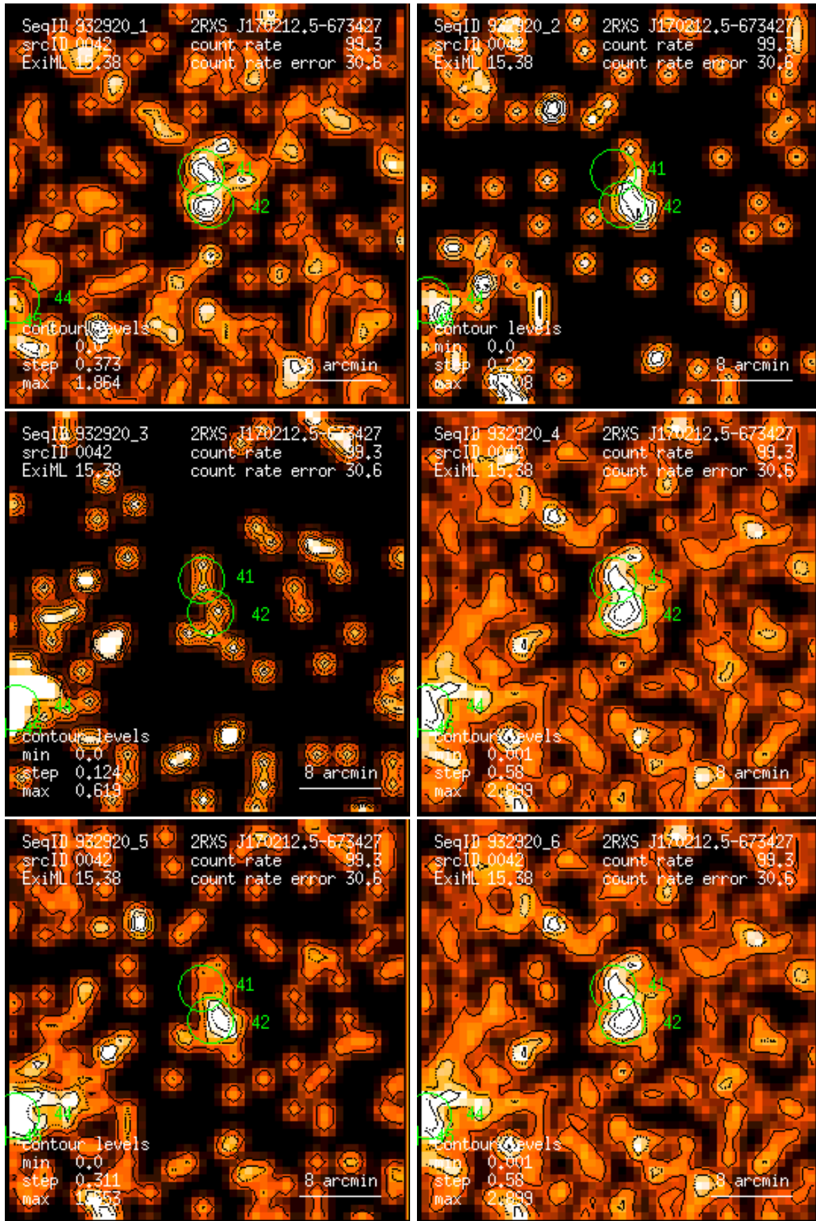
Figure 42: RASS 932920: detection 0042: band rate images, Gaussian filter: (1) PSPC channels 11 – 41, (2) 52 – 90, (3) 91 – 201, (4) 11 – 235, (5) 52 – 201, (6) 11 – 201. Broad band rates in counts/ks. Band rate contour levels in counts/ks/arcmin 2 .
