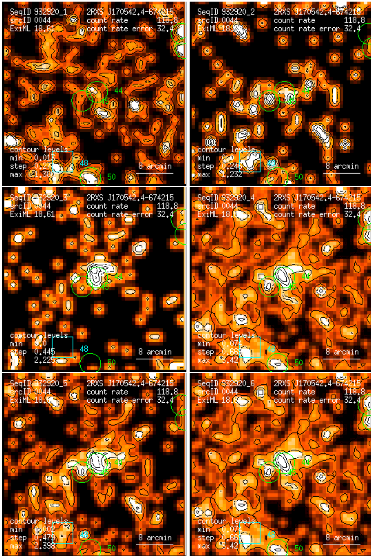
Figure 44: RASS 932920: detection 0044: band rate images, Gaussian filter: (1) PSPC channels 11 – 41, (2) 52 – 90, (3) 91 – 201, (4) 11 – 235, (5) 52 – 201, (6) 11 – 201. Broad band rates in counts/ks. Band rate contour levels in counts/ks/arcmin 2 .
