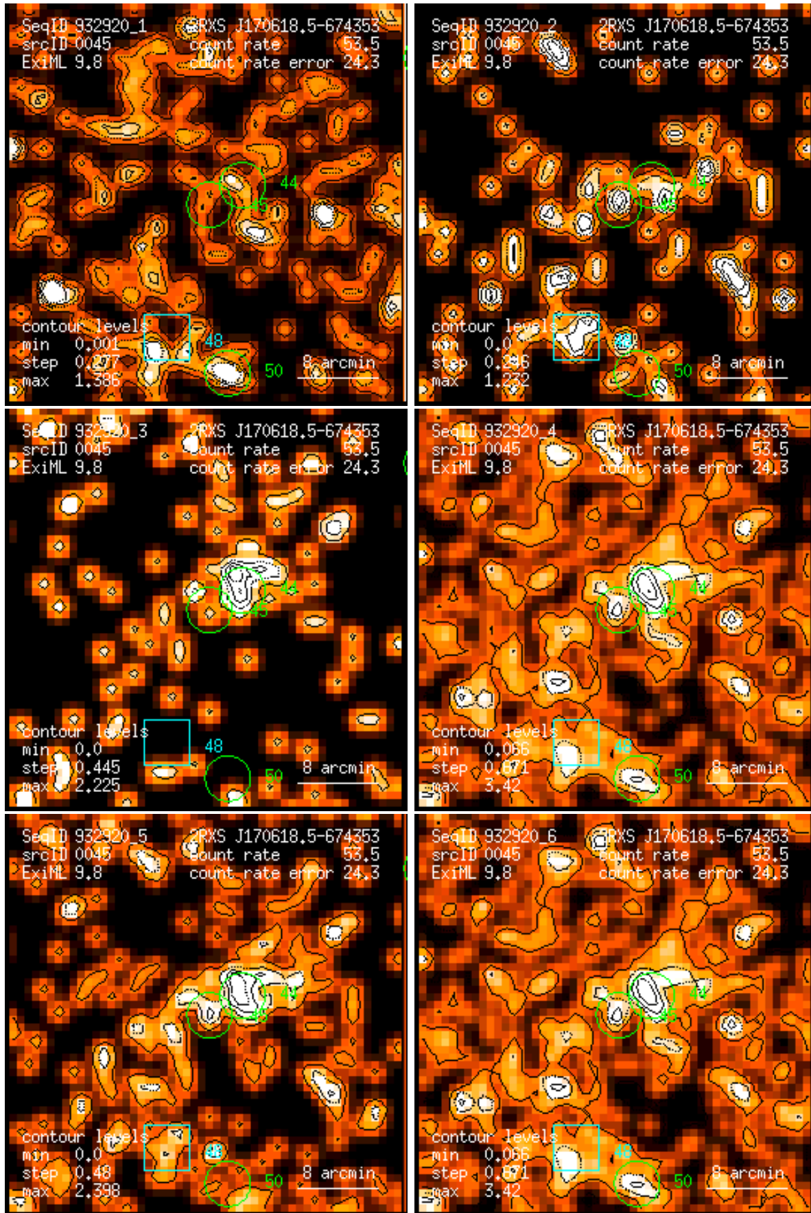
Figure 45: RASS 932920: detection 0045: band rate images, Gaussian filter: (1) PSPC channels 11 – 41, (2) 52 – 90, (3) 91 – 201, (4) 11 – 235, (5) 52 – 201, (6) 11 – 201. Broad band rates in counts/ks. Band rate contour levels in counts/ks/arcmin 2 .
