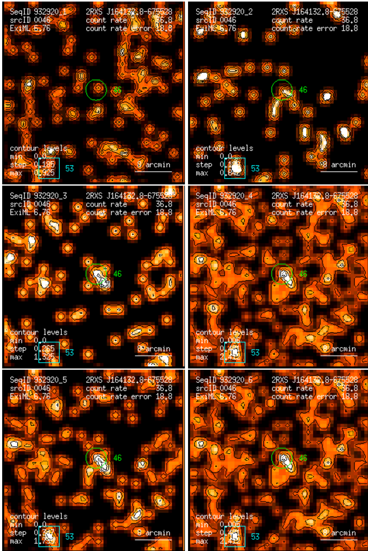
Figure 46: RASS 932920: detection 0046: band rate images, Gaussian filter: (1) PSPC channels 11 – 41, (2) 52 – 90, (3) 91 – 201, (4) 11 – 235, (5) 52 – 201, (6) 11 – 201. Broad band rates in counts/ks. Band rate contour levels in counts/ks/arcmin 2 .
