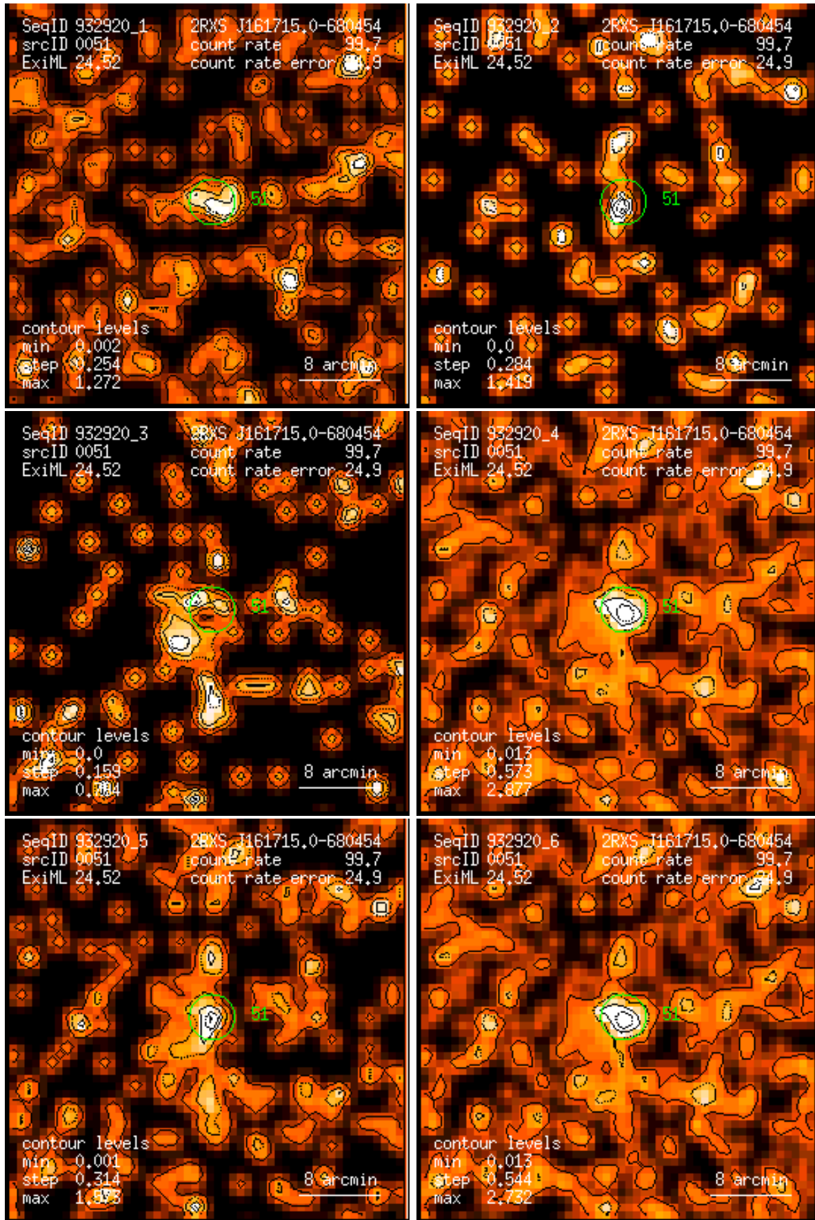
Figure 51: RASS 932920: detection 0051: band rate images, Gaussian filter: (1) PSPC channels 11 – 41, (2) 52 – 90, (3) 91 – 201, (4) 11 – 235, (5) 52 – 201, (6) 11 – 201. Broad band rates in counts/ks. Band rate contour levels in counts/ks/arcmin 2 .
