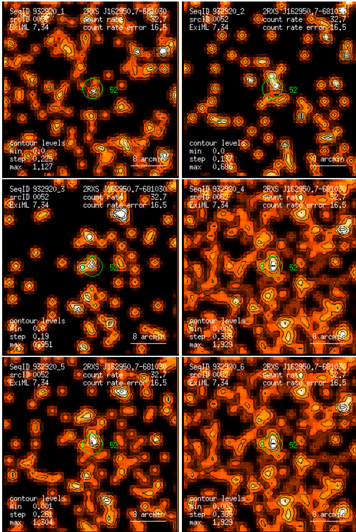
Figure 52: RASS 932920: detection 0052: band rate images, Gaussian filter: (1) PSPC channels 11 – 41, (2) 52 – 90, (3) 91 – 201, (4) 11 – 235, (5) 52 – 201, (6) 11 – 201. Broad band rates in counts/ks. Band rate contour levels in counts/ks/arcmin 2 .
