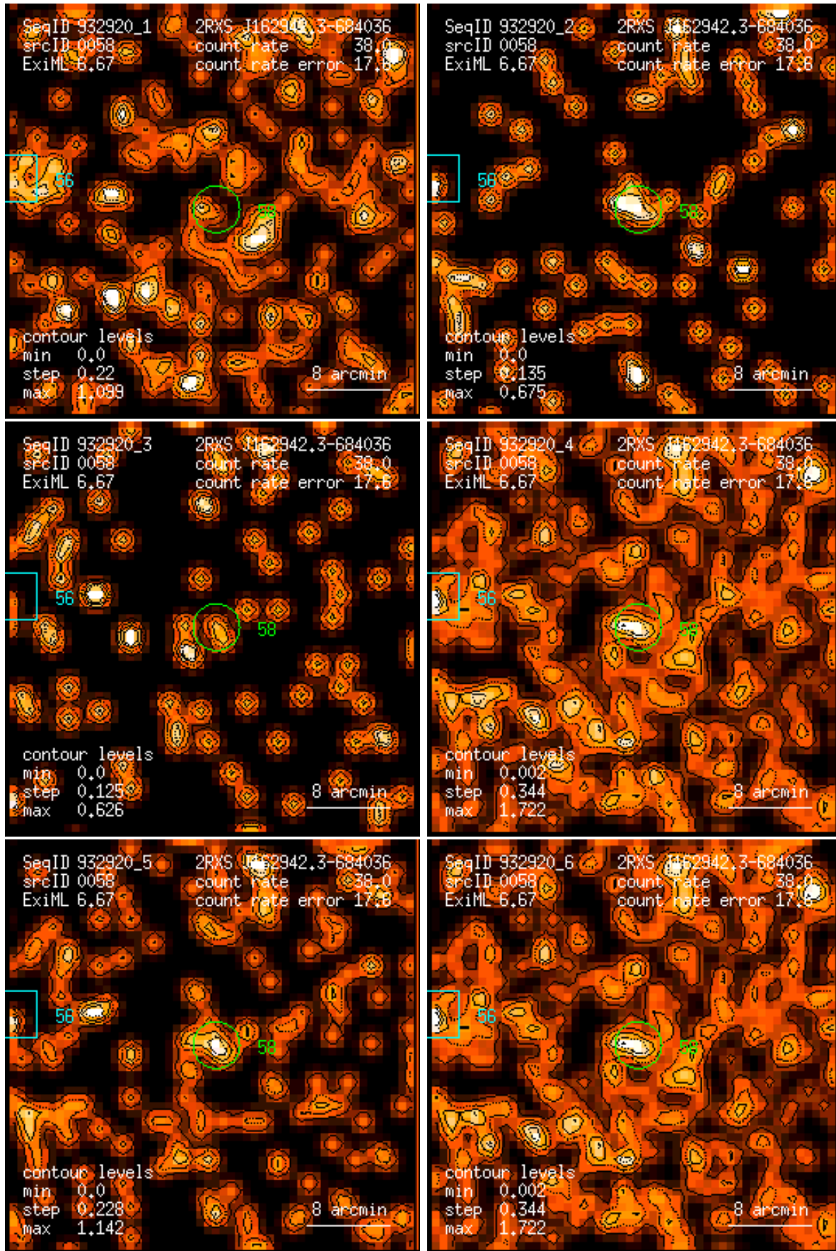
Figure 58: RASS 932920: detection 0058: band rate images, Gaussian filter: (1) PSPC channels 11 – 41, (2) 52 – 90, (3) 91 – 201, (4) 11 – 235, (5) 52 – 201, (6) 11 – 201. Broad band rates in counts/ks. Band rate contour levels in counts/ks/arcmin 2 .
