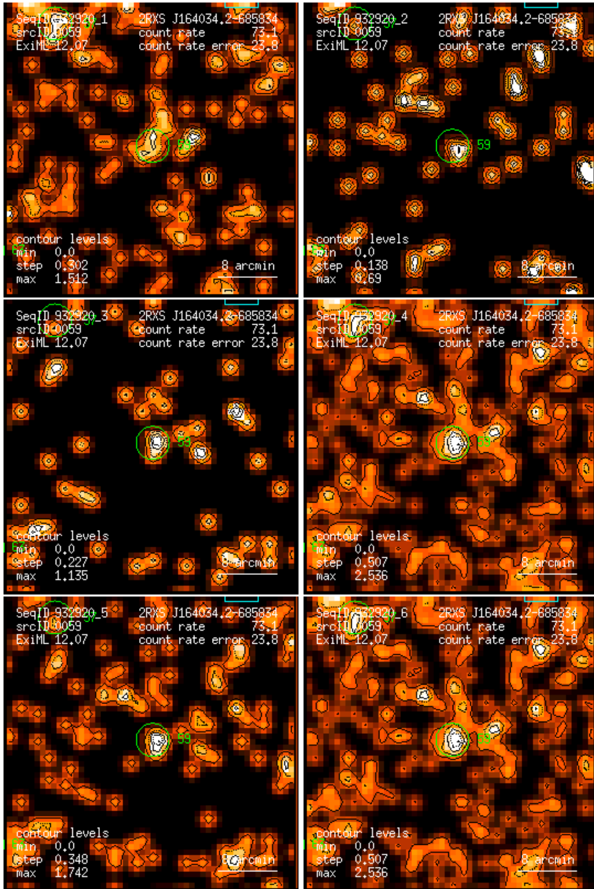
Figure 59: RASS 932920: detection 0059: band rate images, Gaussian filter: (1) PSPC channels 11 – 41, (2) 52 – 90, (3) 91 – 201, (4) 11 – 235, (5) 52 – 201, (6) 11 – 201. Broad band rates in counts/ks. Band rate contour levels in counts/ks/arcmin 2 .
