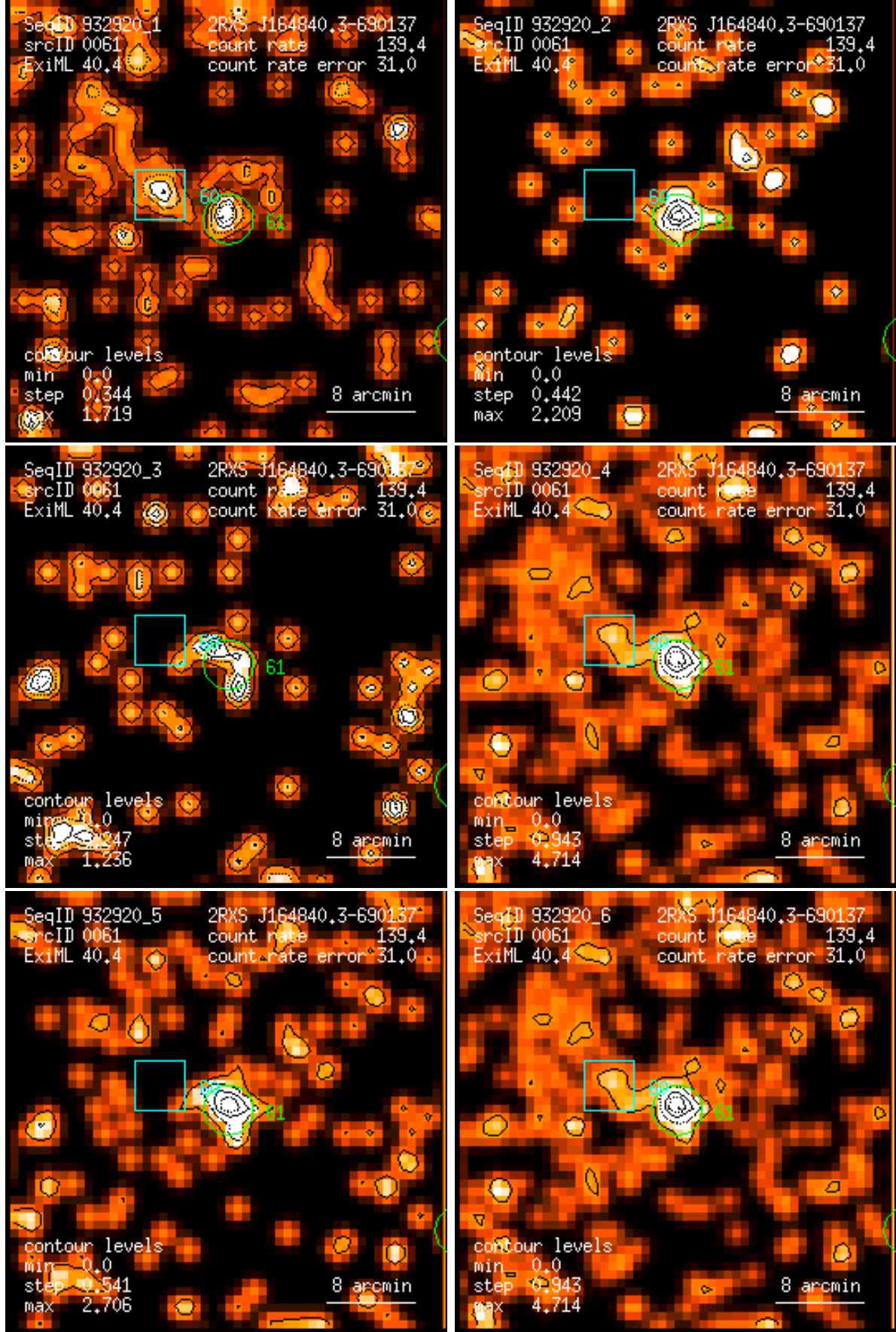
Figure 61: RASS 932920: detection 0061: band rate images, Gaussian filter: (1) PSPC channels 11 – 41, (2) 52 – 90, (3) 91 – 201, (4) 11 – 235, (5) 52 – 201, (6) 11 – 201. Broad band rates in counts/ks. Band rate contour levels in counts/ks/arcmin 2 .
