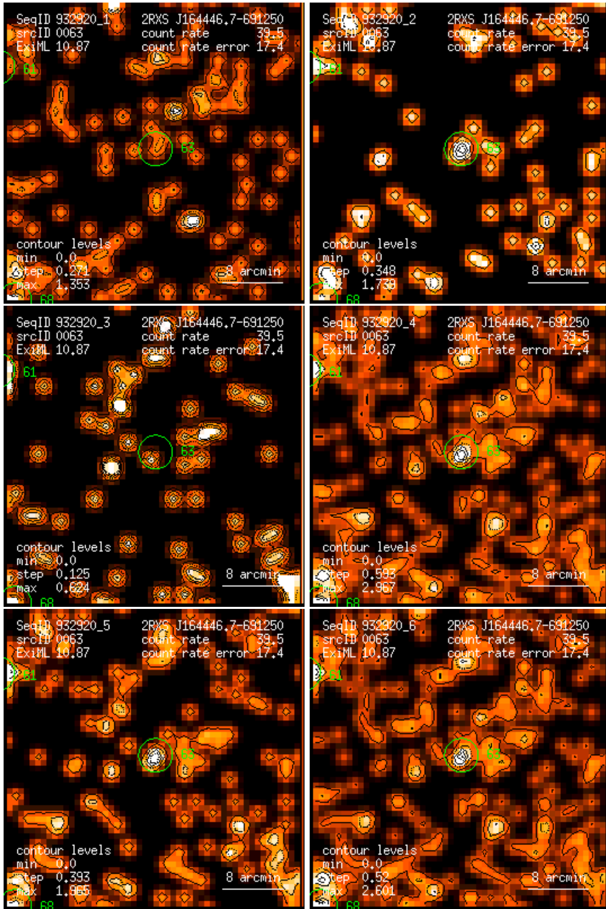
Figure 63: RASS 932920: detection 0063: band rate images, Gaussian filter: (1) PSPC channels 11 – 41, (2) 52 – 90, (3) 91 – 201, (4) 11 – 235, (5) 52 – 201, (6) 11 – 201. Broad band rates in counts/ks. Band rate contour levels in counts/ks/arcmin 2 .
