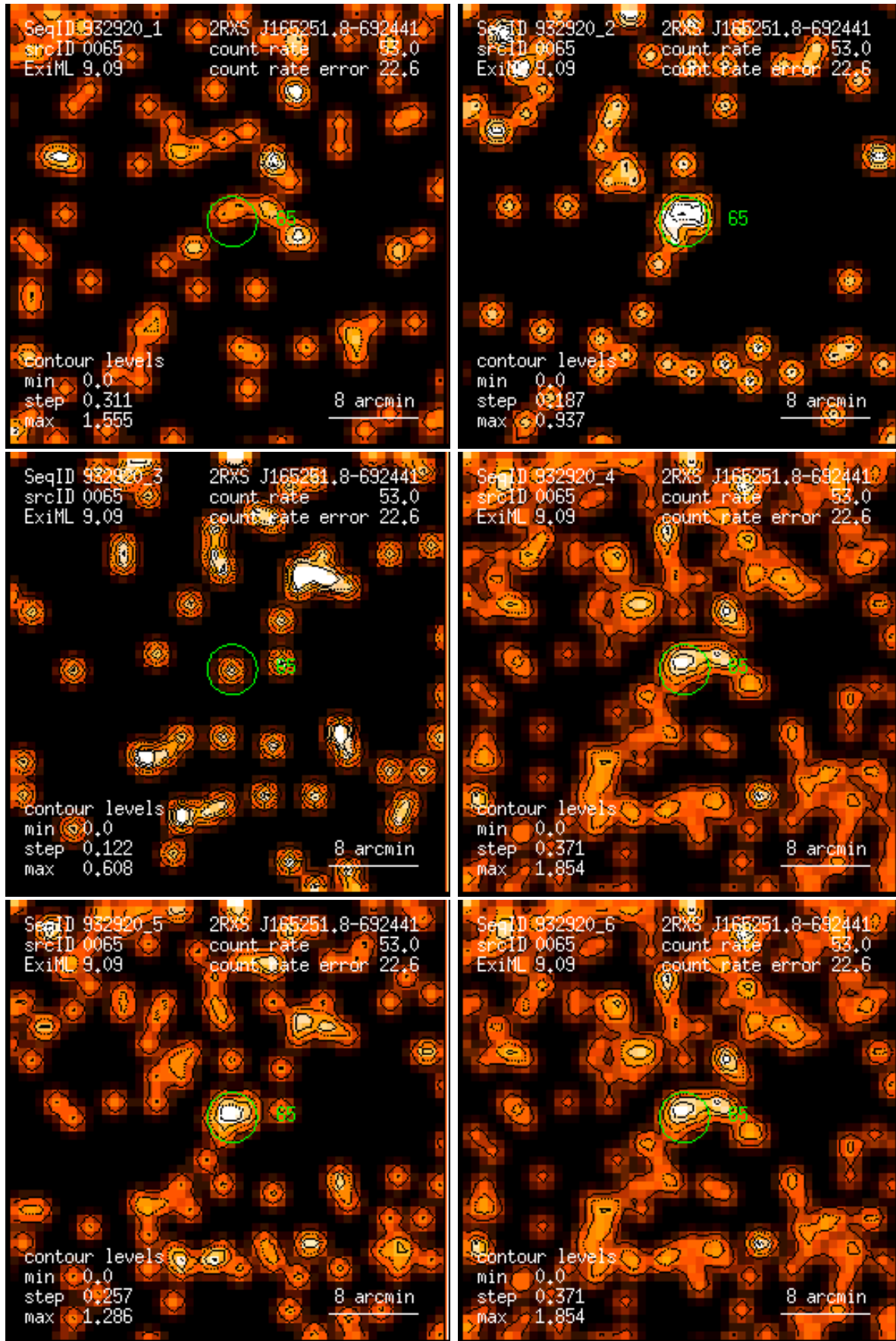
Figure 65: RASS 932920: detection 0065: band rate images, Gaussian filter: (1) PSPC channels 11 – 41, (2) 52 – 90, (3) 91 – 201, (4) 11 – 235, (5) 52 – 201, (6) 11 – 201. Broad band rates in counts/ks. Band rate contour levels in counts/ks/arcmin 2 .
