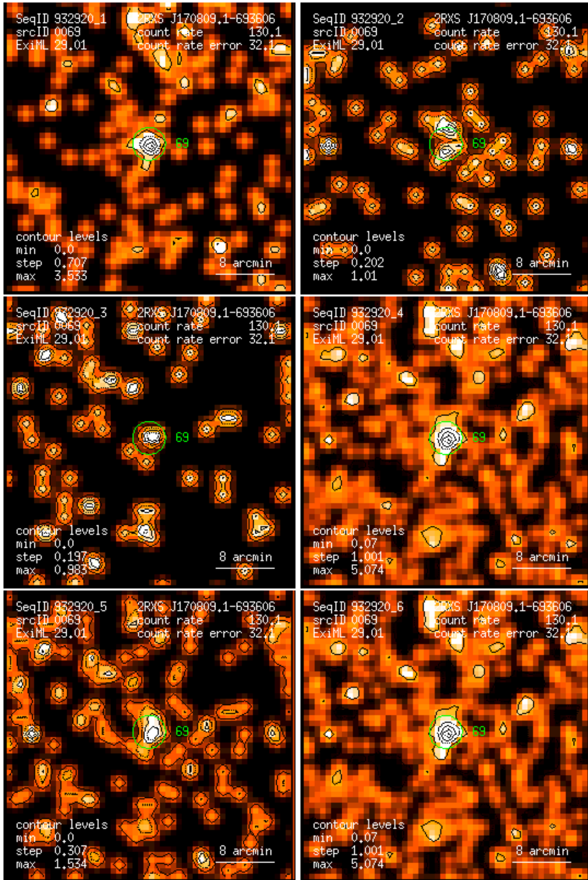
Figure 69: RASS 932920: detection 0069: band rate images, Gaussian filter: (1) PSPC channels 11 – 41, (2) 52 – 90, (3) 91 – 201, (4) 11 – 235, (5) 52 – 201, (6) 11 – 201. Broad band rates in counts/ks. Band rate contour levels in counts/ks/arcmin 2 .
