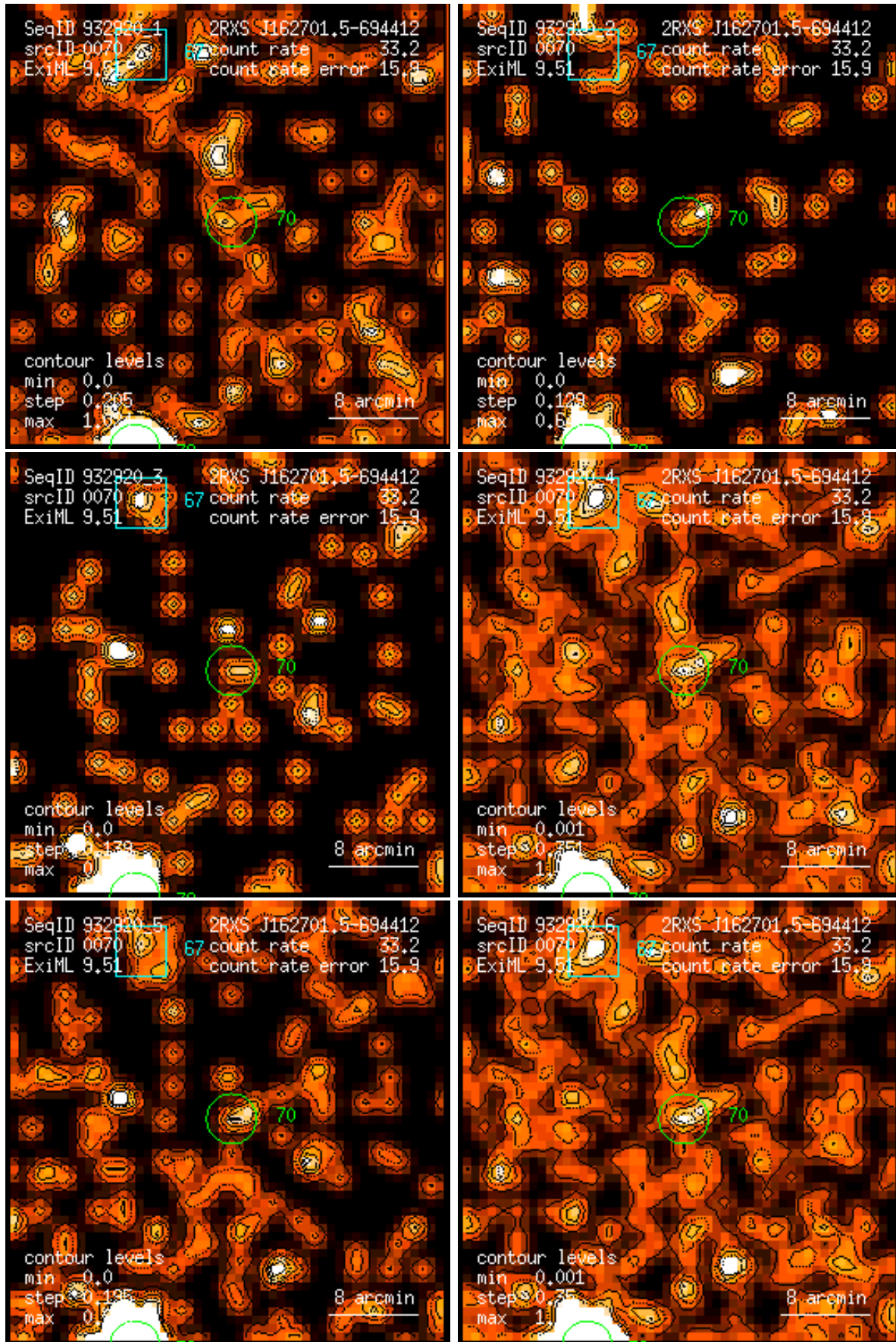
Figure 70: RASS 932920: detection 0070: band rate images, Gaussian filter: (1) PSPC channels 11 – 41, (2) 52 – 90, (3) 91 – 201, (4) 11 – 235, (5) 52 – 201, (6) 11 – 201. Broad band rates in counts/ks. Band rate contour levels in counts/ks/arcmin 2 .
