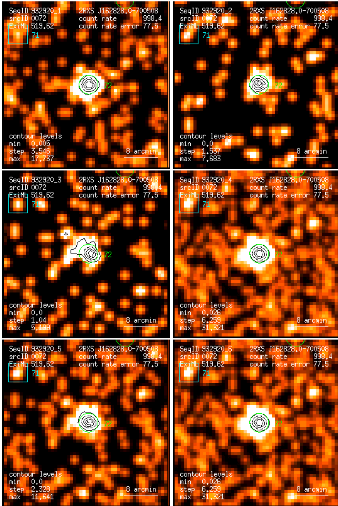
Figure 72: RASS 932920: detection 0072: band rate images, Gaussian filter: (1) PSPC channels 11 – 41, (2) 52 – 90, (3) 91 – 201, (4) 11 – 235, (5) 52 – 201, (6) 11 – 201. Broad band rates in counts/ks. Band rate contour levels in counts/ks/arcmin 2 .
