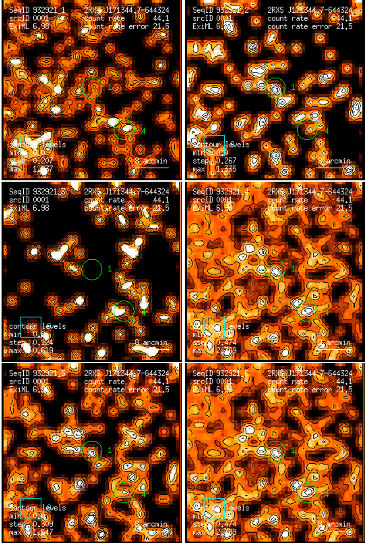
Figure 1: RASS 932921: detection 0001: band rate images, Gaussian filter: (1) PSPC channels 11 – 41, (2) 52 – 90, (3) 91 – 201, (4) 11 – 235, (5) 52 – 201, (6) 11 – 201. Broad band rates in counts/ks. Band rate contour levels in counts/ks/arcmin 2 .
