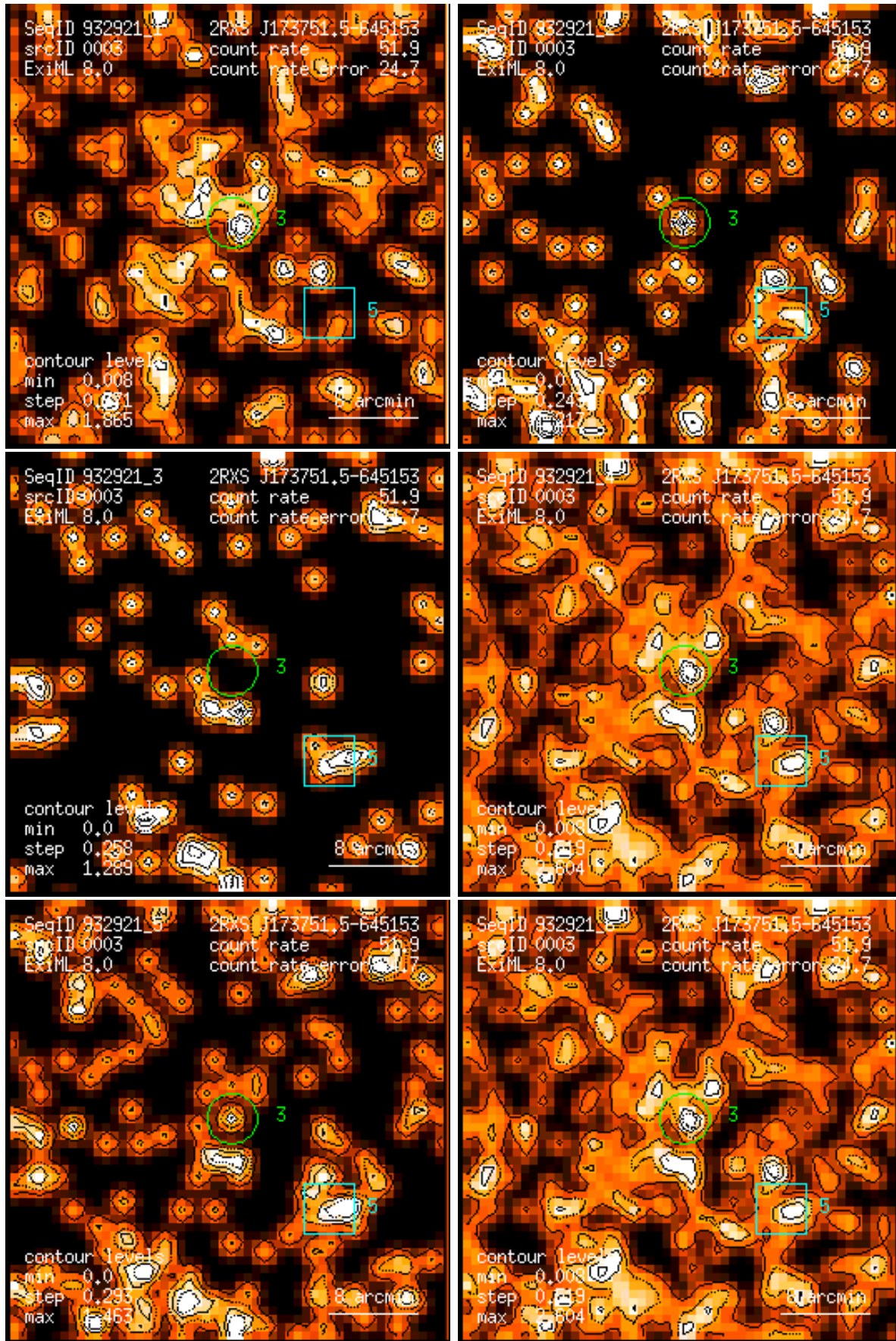
Figure 3: RASS 932921: detection 0003: band rate images, Gaussian filter: (1) PSPC channels 11 – 41, (2) 52 – 90, (3) 91 – 201, (4) 11 – 235, (5) 52 – 201, (6) 11 – 201. Broad band rates in counts/ks. Band rate contour levels in counts/ks/arcmin 2 .
