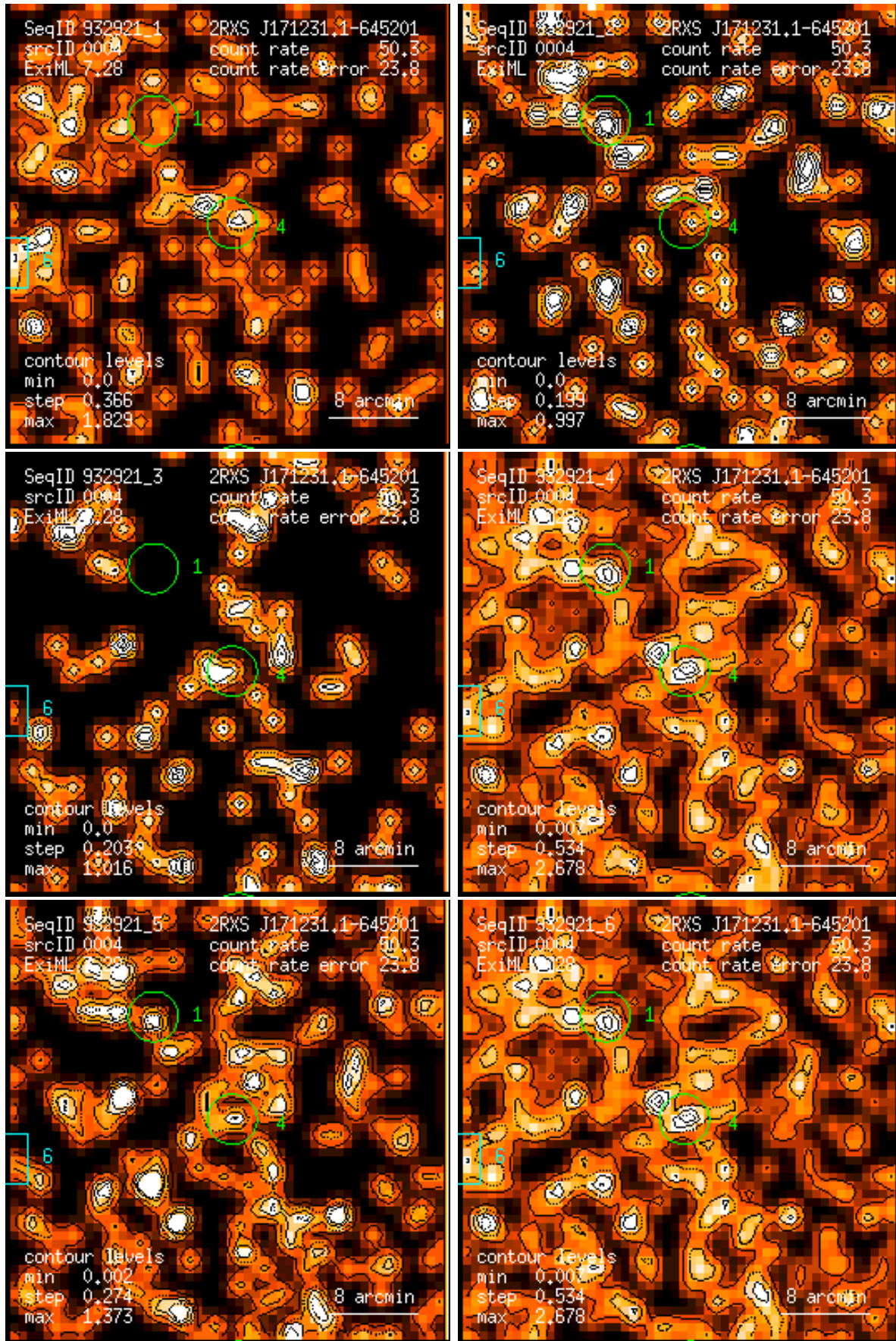
Figure 4: RASS 932921: detection 0004: band rate images, Gaussian filter: (1) PSPC channels 11 – 41, (2) 52 – 90, (3) 91 – 201, (4) 11 – 235, (5) 52 – 201, (6) 11 – 201. Broad band rates in counts/ks. Band rate contour levels in counts/ks/arcmin 2 .
