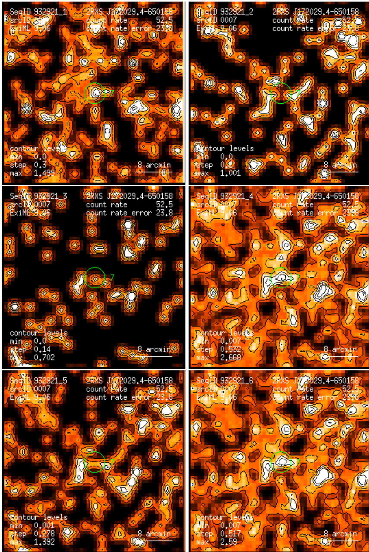
Figure 7: RASS 932921: detection 0007: band rate images, Gaussian filter: (1) PSPC channels 11 – 41, (2) 52 – 90, (3) 91 – 201, (4) 11 – 235, (5) 52 – 201, (6) 11 – 201. Broad band rates in counts/ks. Band rate contour levels in counts/ks/arcmin 2 .
