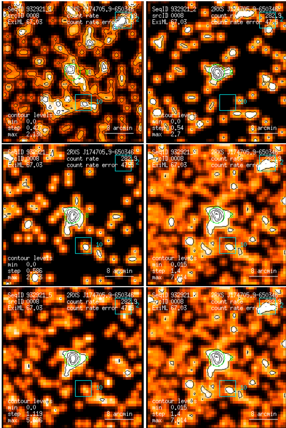
Figure 8: RASS 932921: detection 0008: band rate images, Gaussian filter: (1) PSPC channels 11 – 41, (2) 52 – 90, (3) 91 – 201, (4) 11 – 235, (5) 52 – 201, (6) 11 – 201. Broad band rates in counts/ks. Band rate contour levels in counts/ks/arcmin 2 .
