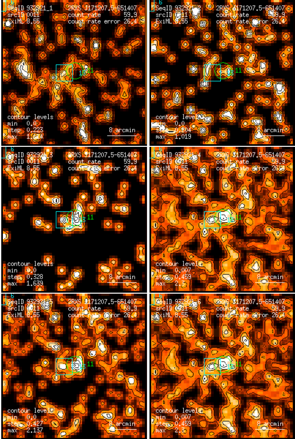
Figure 11: RASS 932921: detection 0011: band rate images, Gaussian filter: (1) PSPC channels 11 – 41, (2) 52 – 90, (3) 91 – 201, (4) 11 – 235, (5) 52 – 201, (6) 11 – 201. Broad band rates in counts/ks. Band rate contour levels in counts/ks/arcmin 2 .
