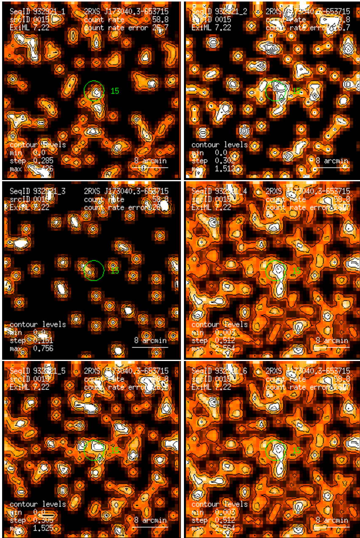
Figure 15: RASS 932921: detection 0015: band rate images, Gaussian filter: (1) PSPC channels 11 – 41, (2) 52 – 90, (3) 91 – 201, (4) 11 – 235, (5) 52 – 201, (6) 11 – 201. Broad band rates in counts/ks. Band rate contour levels in counts/ks/arcmin 2 .
