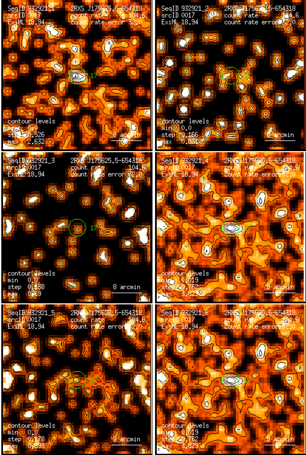
Figure 17: RASS 932921: detection 0017: band rate images, Gaussian filter: (1) PSPC channels 11 – 41, (2) 52 – 90, (3) 91 – 201, (4) 11 – 235, (5) 52 – 201, (6) 11 – 201. Broad band rates in counts/ks. Band rate contour levels in counts/ks/arcmin 2 .
