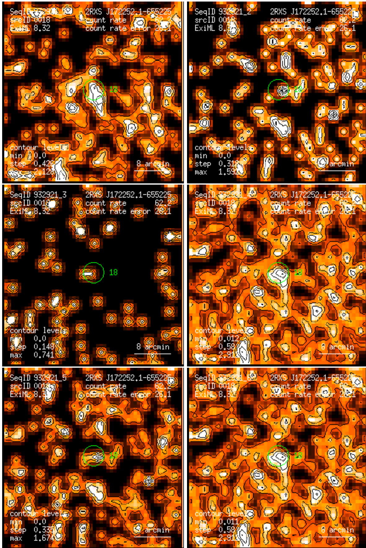
Figure 18: RASS 932921: detection 0018: band rate images, Gaussian filter: (1) PSPC channels 11 – 41, (2) 52 – 90, (3) 91 – 201, (4) 11 – 235, (5) 52 – 201, (6) 11 – 201. Broad band rates in counts/ks. Band rate contour levels in counts/ks/arcmin 2 .
