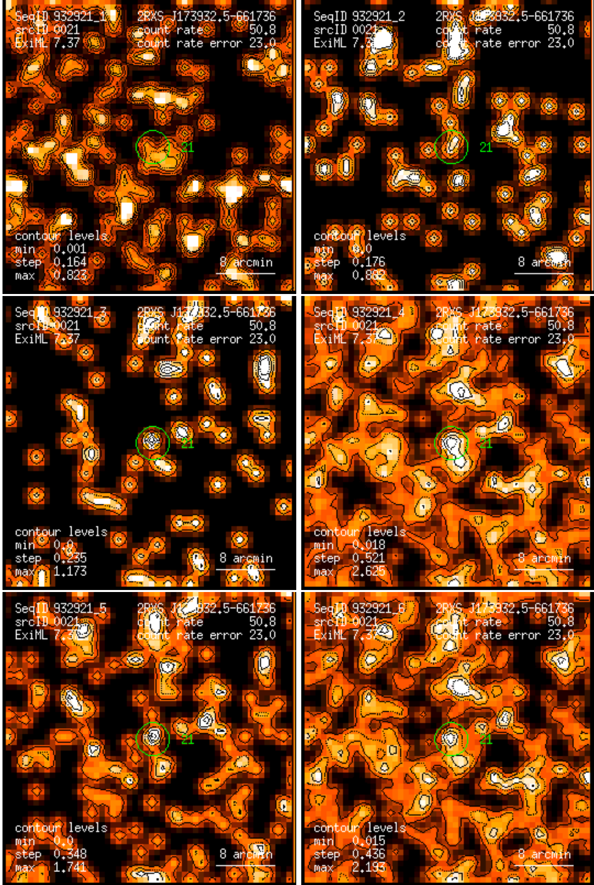
Figure 21: RASS 932921: detection 0021: band rate images, Gaussian filter: (1) PSPC channels 11 – 41, (2) 52 – 90, (3) 91 – 201, (4) 11 – 235, (5) 52 – 201, (6) 11 – 201. Broad band rates in counts/ks. Band rate contour levels in counts/ks/arcmin 2 .
