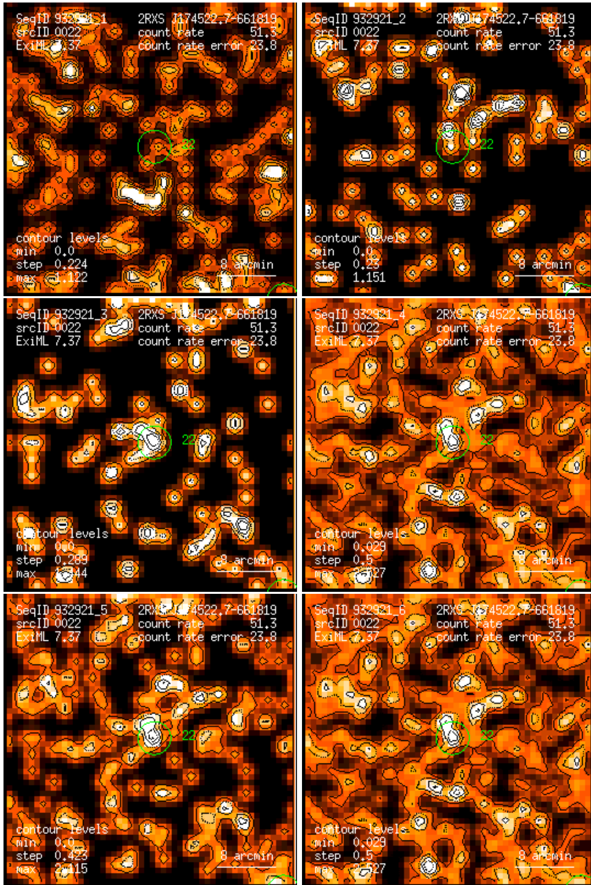
Figure 22: RASS 932921: detection 0022: band rate images, Gaussian filter: (1) PSPC channels 11 – 41, (2) 52 – 90, (3) 91 – 201, (4) 11 – 235, (5) 52 – 201, (6) 11 – 201. Broad band rates in counts/ks. Band rate contour levels in counts/ks/arcmin 2 .
