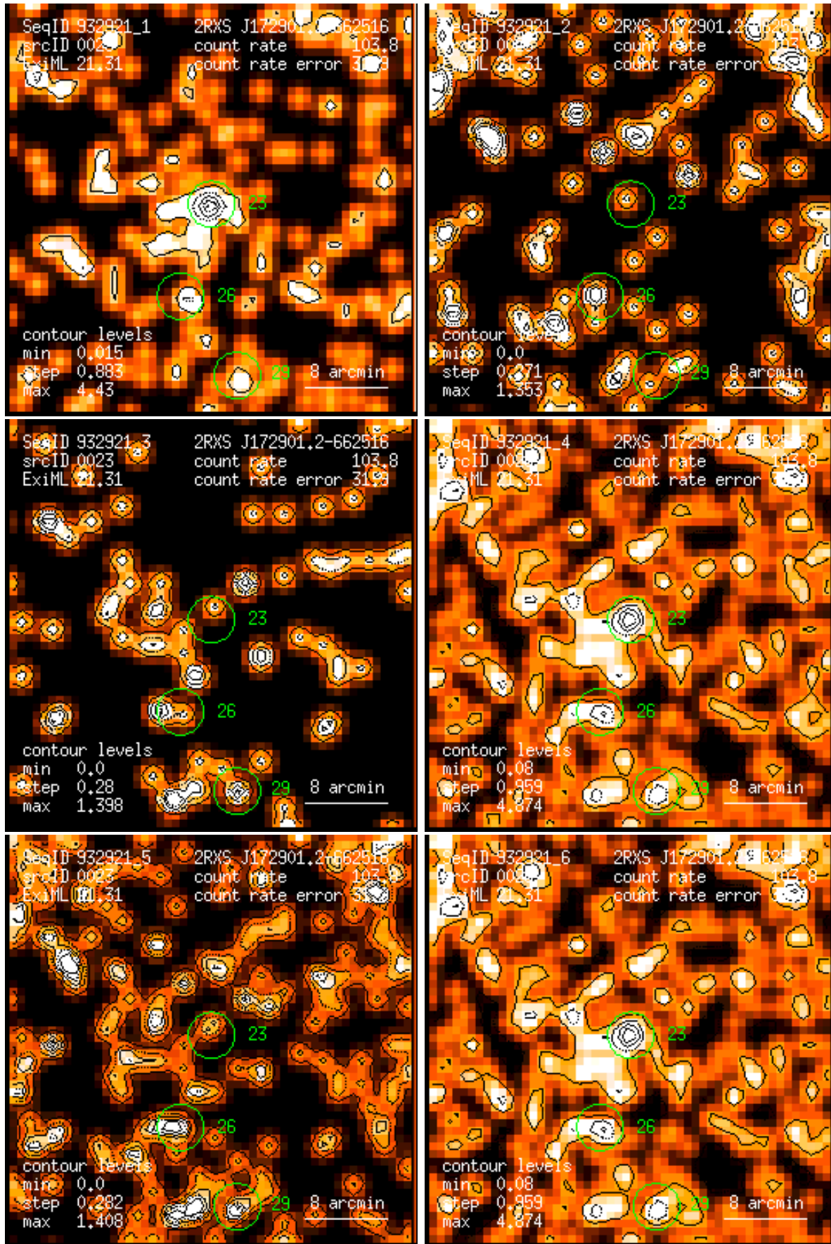
Figure 23: RASS 932921: detection 0023: band rate images, Gaussian filter: (1) PSPC channels 11 – 41, (2) 52 – 90, (3) 91 – 201, (4) 11 – 235, (5) 52 – 201, (6) 11 – 201. Broad band rates in counts/ks. Band rate contour levels in counts/ks/arcmin 2 .
