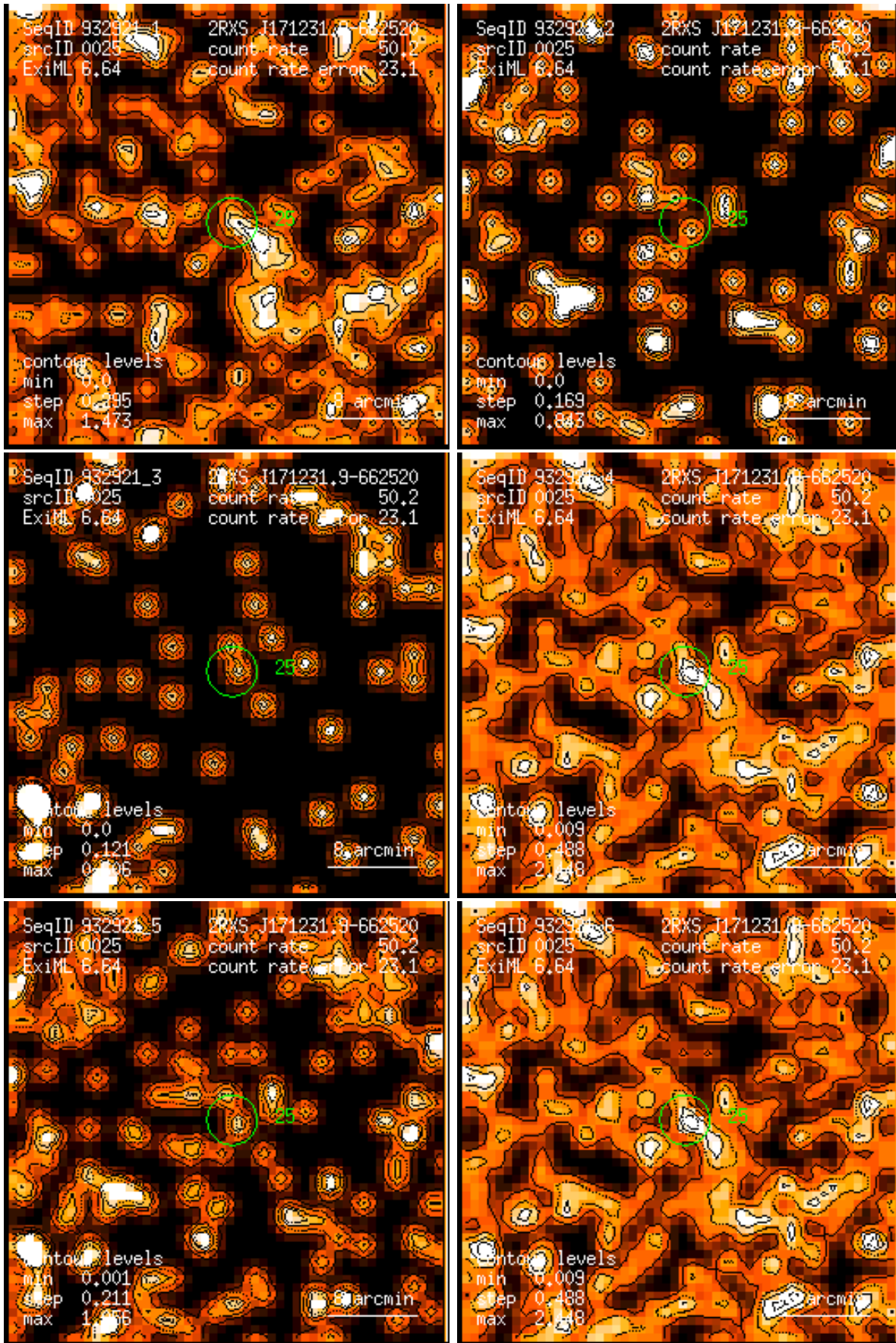
Figure 25: RASS 932921: detection 0025: band rate images, Gaussian filter: (1) PSPC channels 11 – 41, (2) 52 – 90, (3) 91 – 201, (4) 11 – 235, (5) 52 – 201, (6) 11 – 201. Broad band rates in counts/ks. Band rate contour levels in counts/ks/arcmin 2 .
