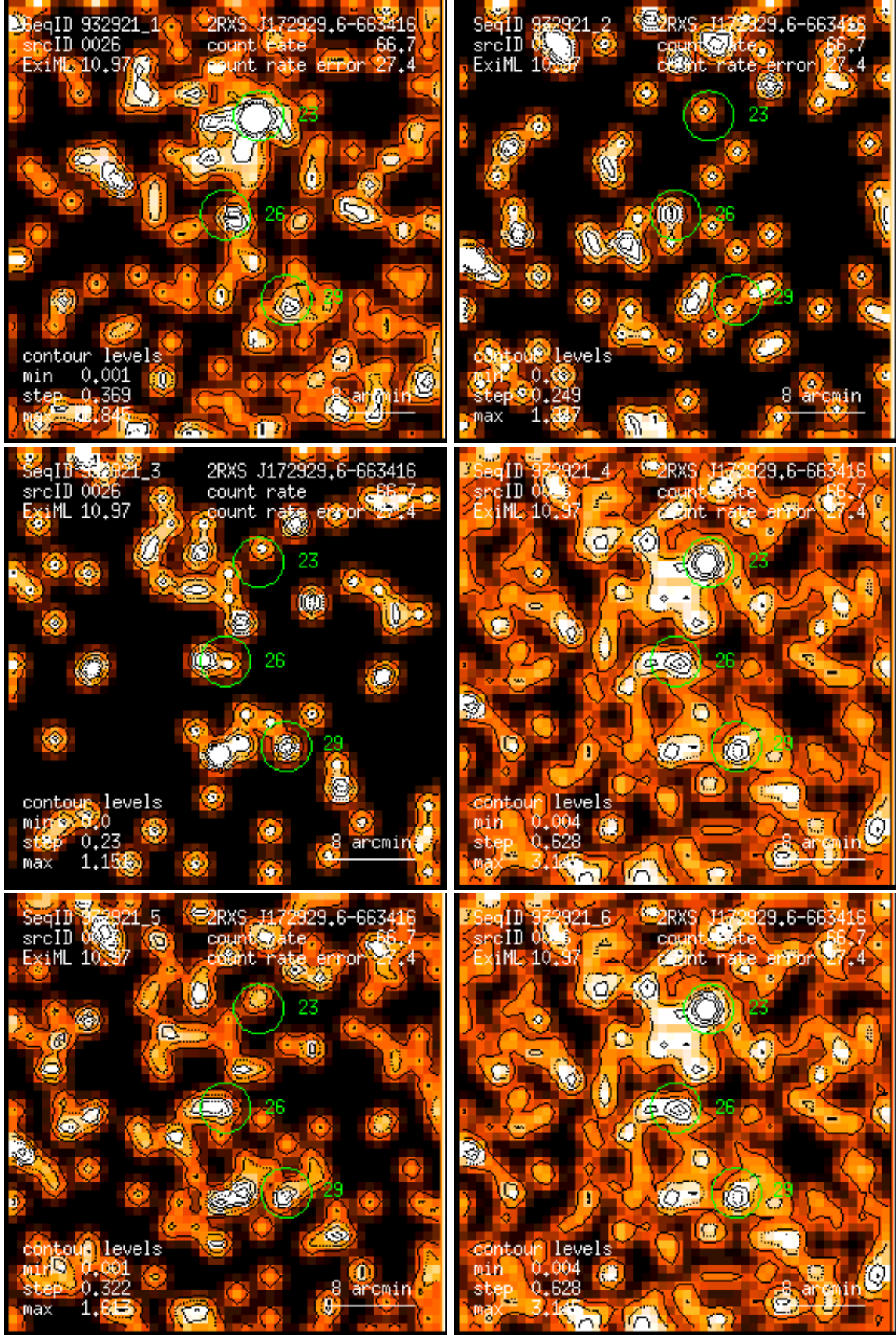
Figure 26: RASS 932921: detection 0026: band rate images, Gaussian filter: (1) PSPC channels 11 – 41, (2) 52 – 90, (3) 91 – 201, (4) 11 – 235, (5) 52 – 201, (6) 11 – 201. Broad band rates in counts/ks. Band rate contour levels in counts/ks/arcmin 2 .
