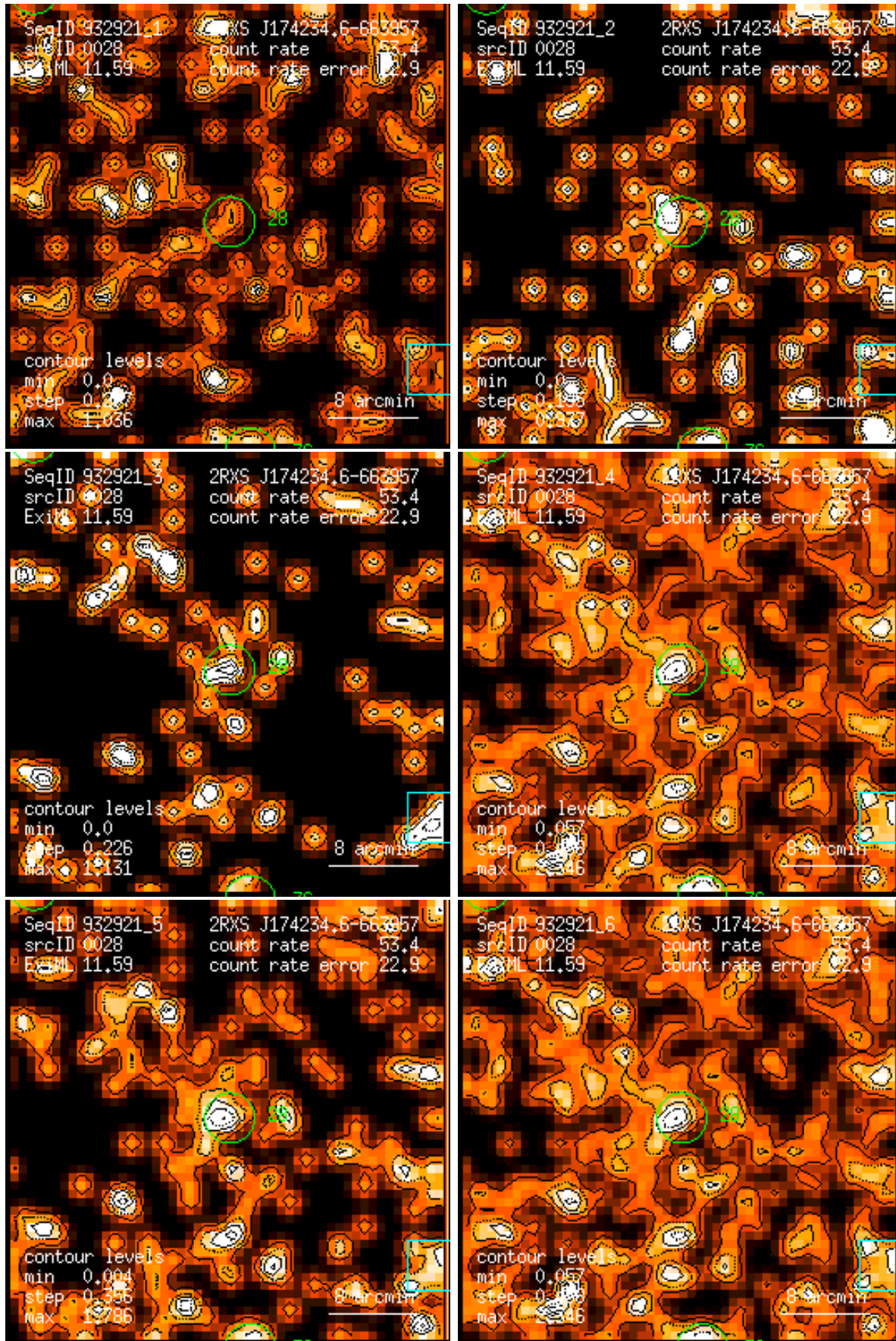
Figure 28: RASS 932921: detection 0028: band rate images, Gaussian filter: (1) PSPC channels 11 – 41, (2) 52 – 90, (3) 91 – 201, (4) 11 – 235, (5) 52 – 201, (6) 11 – 201. Broad band rates in counts/ks. Band rate contour levels in counts/ks/arcmin 2 .
