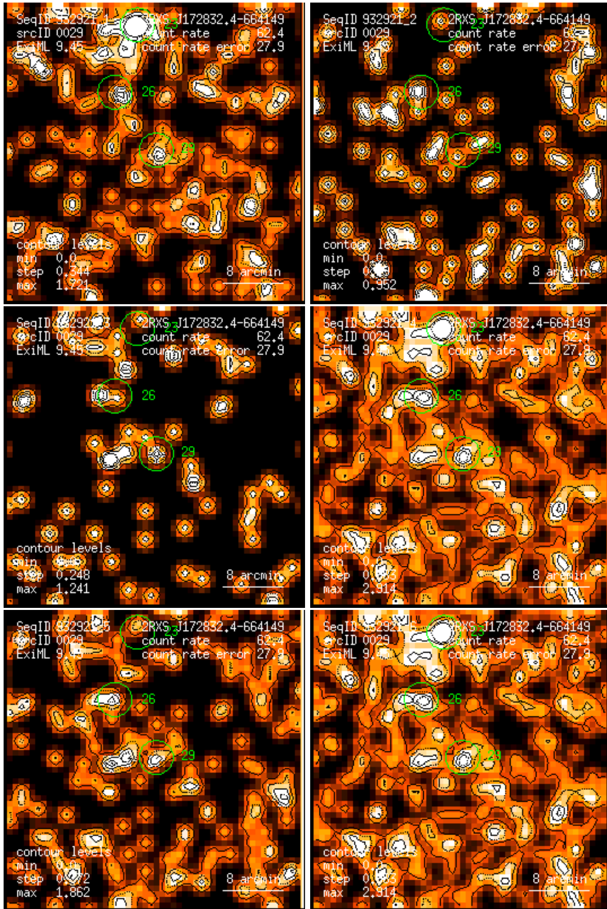
Figure 29: RASS 932921: detection 0029: band rate images, Gaussian filter: (1) PSPC channels 11 – 41, (2) 52 – 90, (3) 91 – 201, (4) 11 – 235, (5) 52 – 201, (6) 11 – 201. Broad band rates in counts/ks. Band rate contour levels in counts/ks/arcmin 2 .
