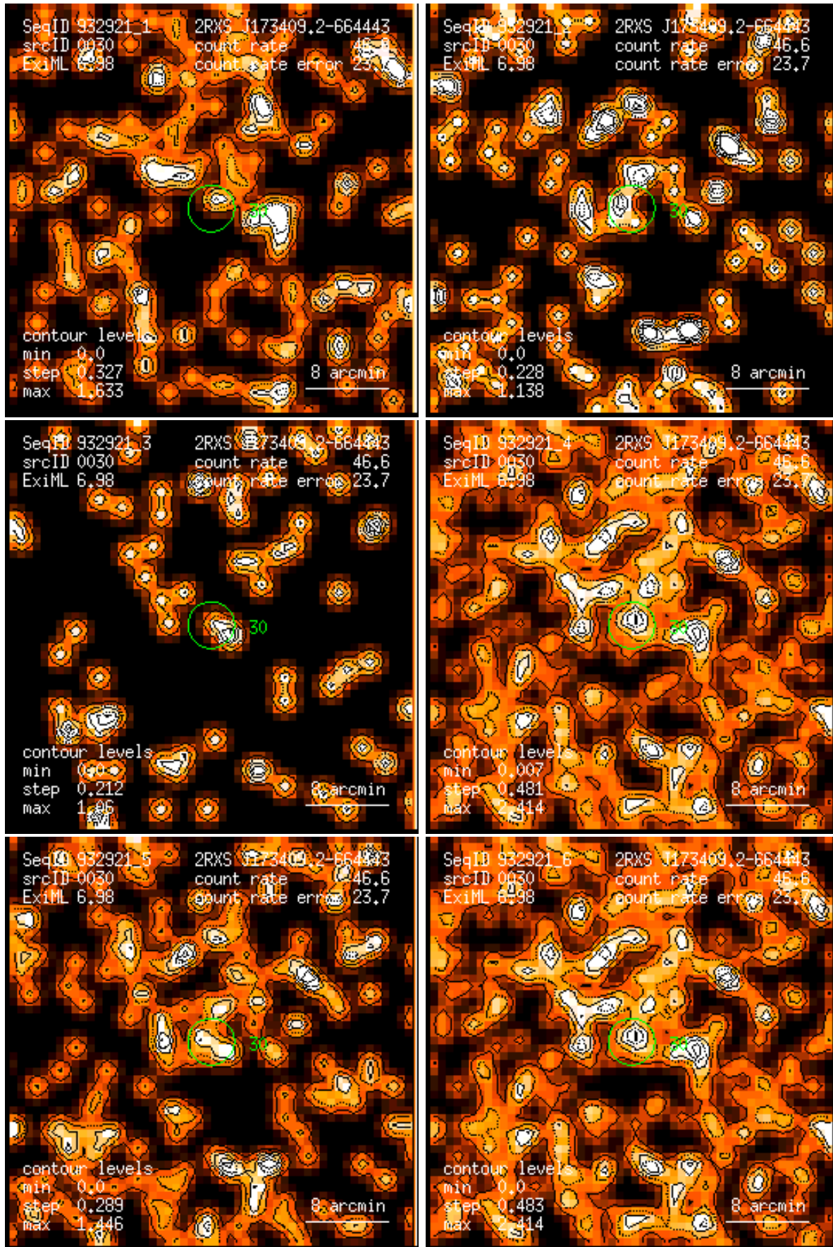
Figure 30: RASS 932921: detection 0030: band rate images, Gaussian filter: (1) PSPC channels 11 – 41, (2) 52 – 90, (3) 91 – 201, (4) 11 – 235, (5) 52 – 201, (6) 11 – 201. Broad band rates in counts/ks. Band rate contour levels in counts/ks/arcmin 2 .
