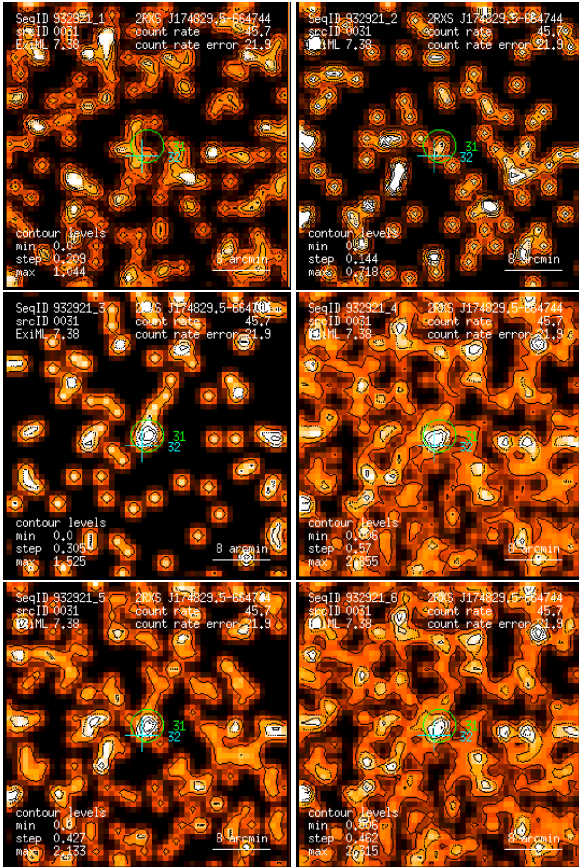
Figure 31: RASS 932921: detection 0031: band rate images, Gaussian filter: (1) PSPC channels 11 – 41, (2) 52 – 90, (3) 91 – 201, (4) 11 – 235, (5) 52 – 201, (6) 11 – 201. Broad band rates in counts/ks. Band rate contour levels in counts/ks/arcmin 2 .
