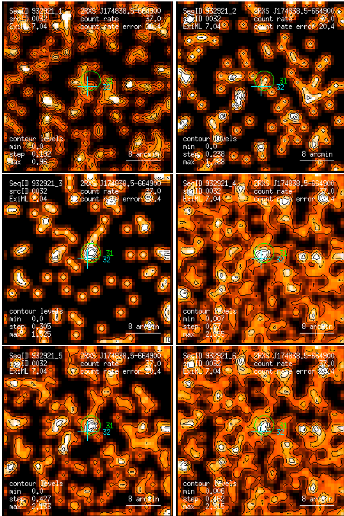
Figure 32: RASS 932921: detection 0032: band rate images, Gaussian filter: (1) PSPC channels 11 – 41, (2) 52 – 90, (3) 91 – 201, (4) 11 – 235, (5) 52 – 201, (6) 11 – 201. Broad band rates in counts/ks. Band rate contour levels in counts/ks/arcmin 2 .
