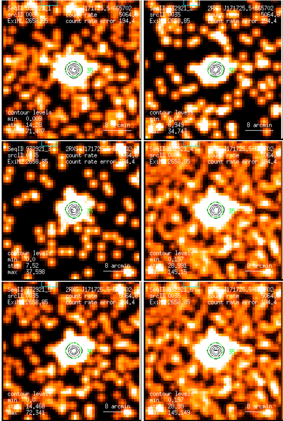
Figure 35: RASS 932921: detection 0035: band rate images, Gaussian filter: (1) PSPC channels 11 – 41, (2) 52 – 90, (3) 91 – 201, (4) 11 – 235, (5) 52 – 201, (6) 11 – 201. Broad band rates in counts/ks. Band rate contour levels in counts/ks/arcmin 2 .
