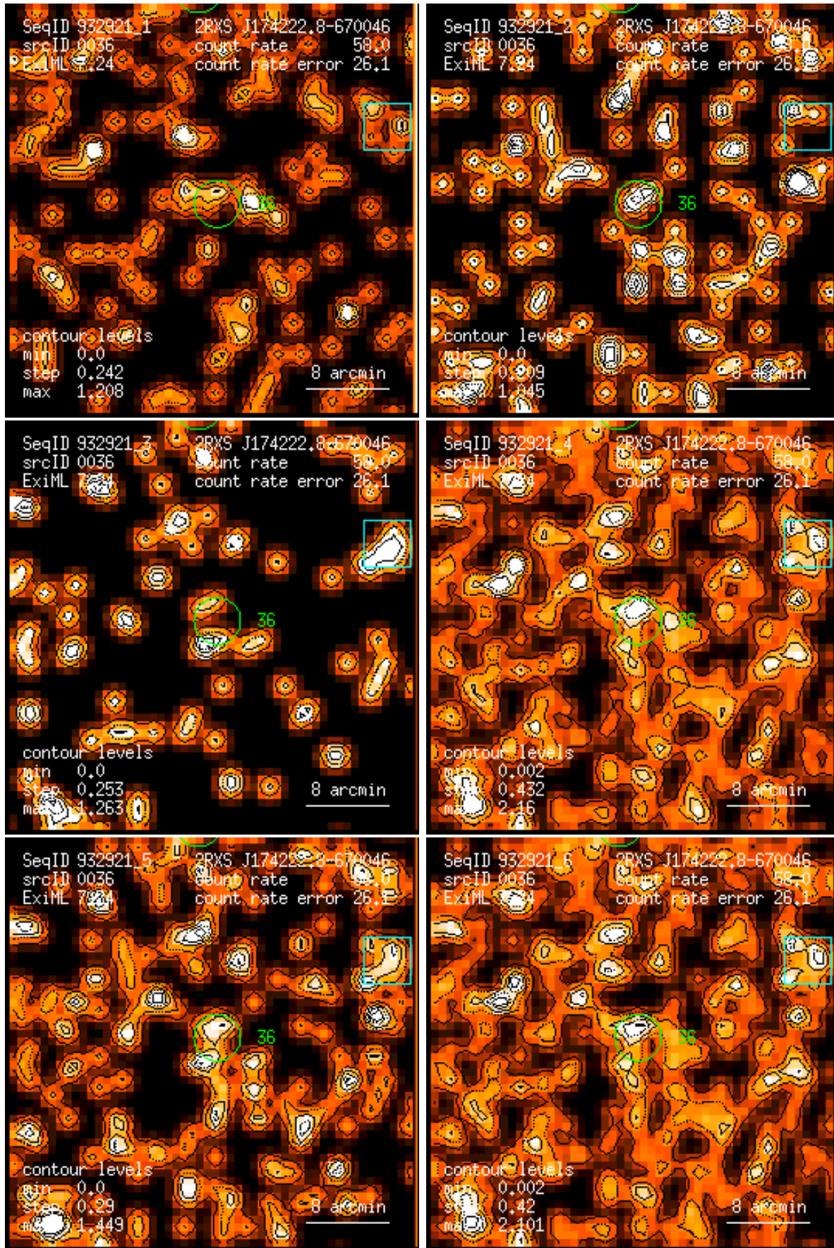
Figure 36: RASS 932921: detection 0036: band rate images, Gaussian filter: (1) PSPC channels 11 – 41, (2) 52 – 90, (3) 91 – 201, (4) 11 – 235, (5) 52 – 201, (6) 11 – 201. Broad band rates in counts/ks. Band rate contour levels in counts/ks/arcmin 2 .
