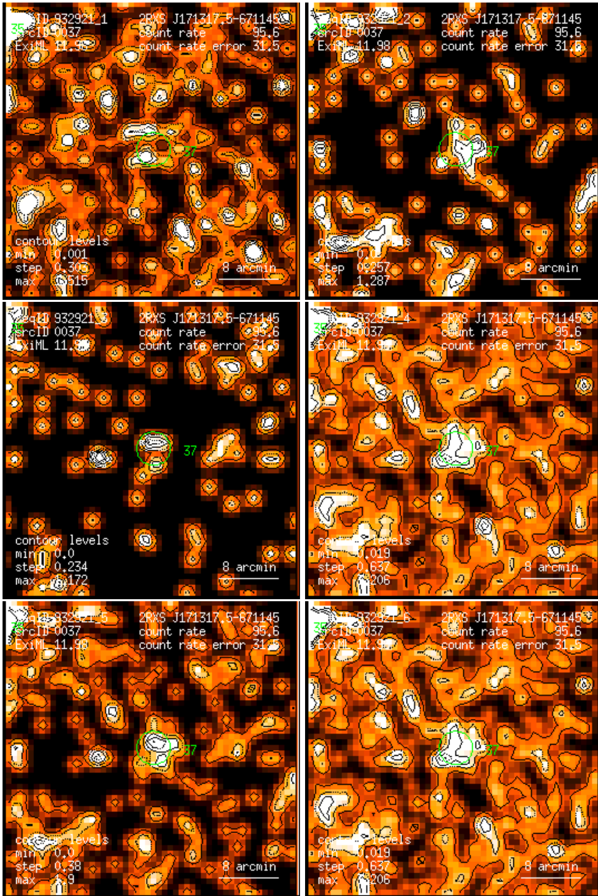
Figure 37: RASS 932921: detection 0037: band rate images, Gaussian filter: (1) PSPC channels 11 – 41, (2) 52 – 90, (3) 91 – 201, (4) 11 – 235, (5) 52 – 201, (6) 11 – 201. Broad band rates in counts/ks. Band rate contour levels in counts/ks/arcmin 2 .
