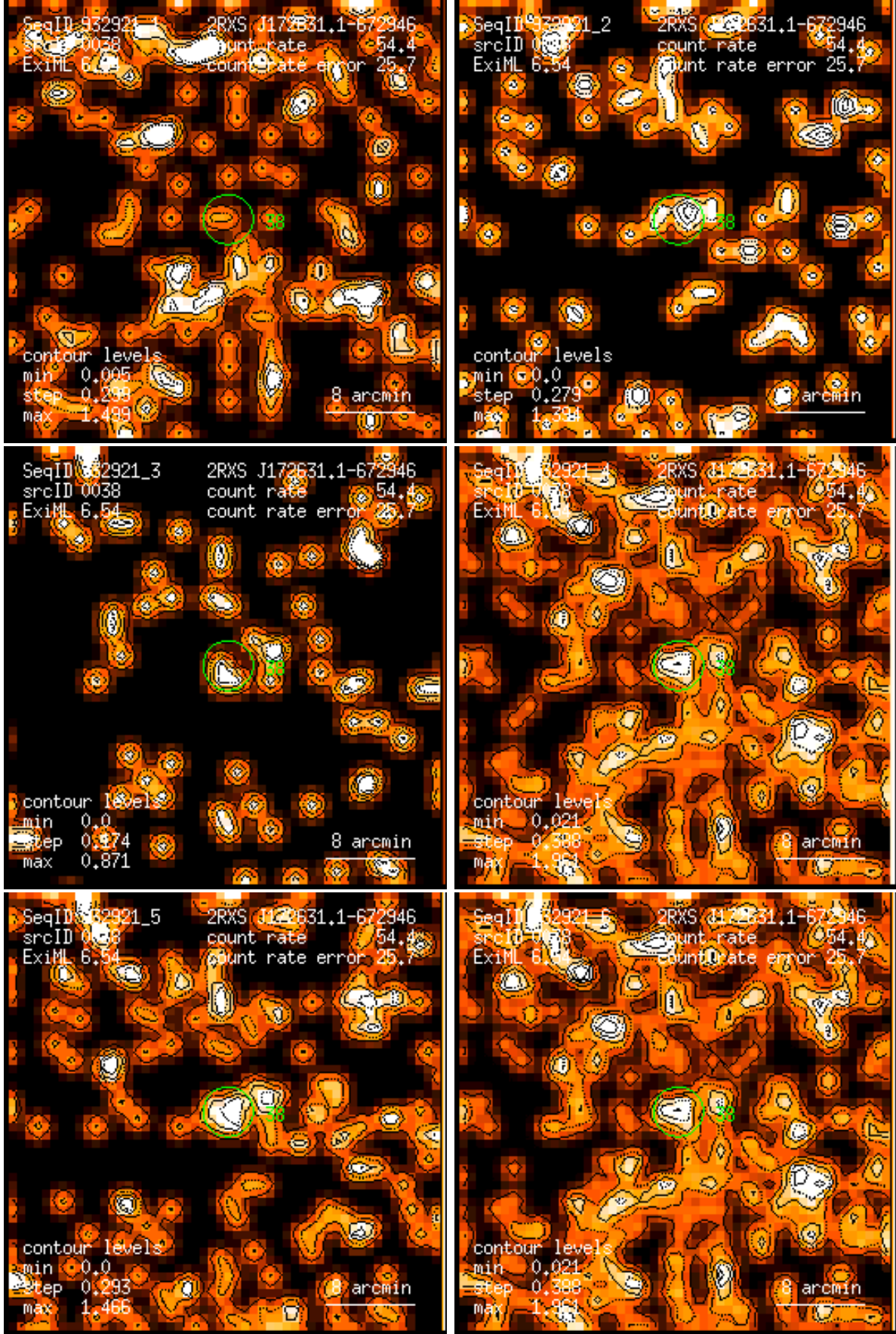
Figure 38: RASS 932921: detection 0038: band rate images, Gaussian filter: (1) PSPC channels 11 – 41, (2) 52 – 90, (3) 91 – 201, (4) 11 – 235, (5) 52 – 201, (6) 11 – 201. Broad band rates in counts/ks. Band rate contour levels in counts/ks/arcmin 2 .
