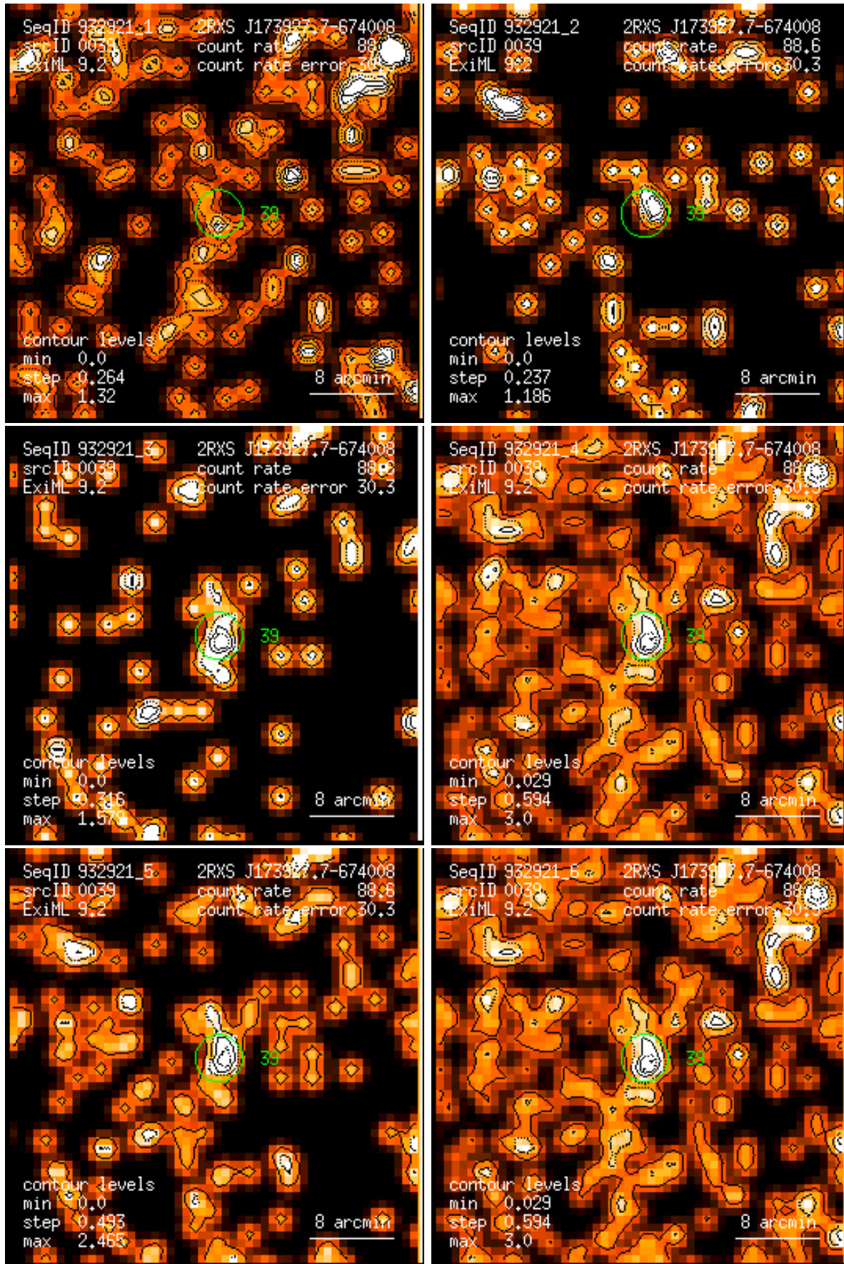
Figure 39: RASS 932921: detection 0039: band rate images, Gaussian filter: (1) PSPC channels 11 – 41, (2) 52 – 90, (3) 91 – 201, (4) 11 – 235, (5) 52 – 201, (6) 11 – 201. Broad band rates in counts/ks. Band rate contour levels in counts/ks/arcmin 2 .
