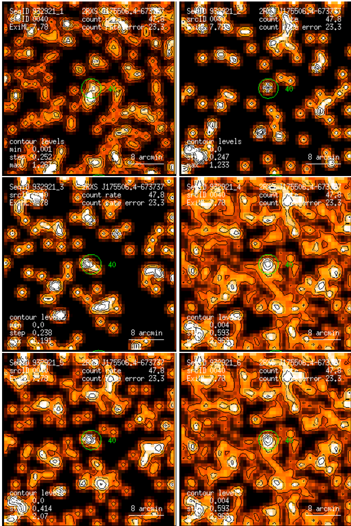
Figure 40: RASS 932921: detection 0040: band rate images, Gaussian filter: (1) PSPC channels 11 – 41, (2) 52 – 90, (3) 91 – 201, (4) 11 – 235, (5) 52 – 201, (6) 11 – 201. Broad band rates in counts/ks. Band rate contour levels in counts/ks/arcmin 2 .
