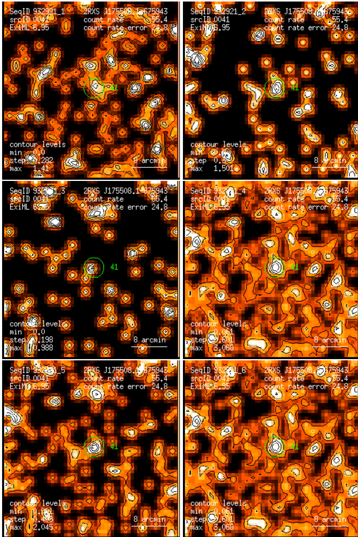
Figure 41: RASS 932921: detection 0041: band rate images, Gaussian filter: (1) PSPC channels 11 – 41, (2) 52 – 90, (3) 91 – 201, (4) 11 – 235, (5) 52 – 201, (6) 11 – 201. Broad band rates in counts/ks. Band rate contour levels in counts/ks/arcmin 2 .
