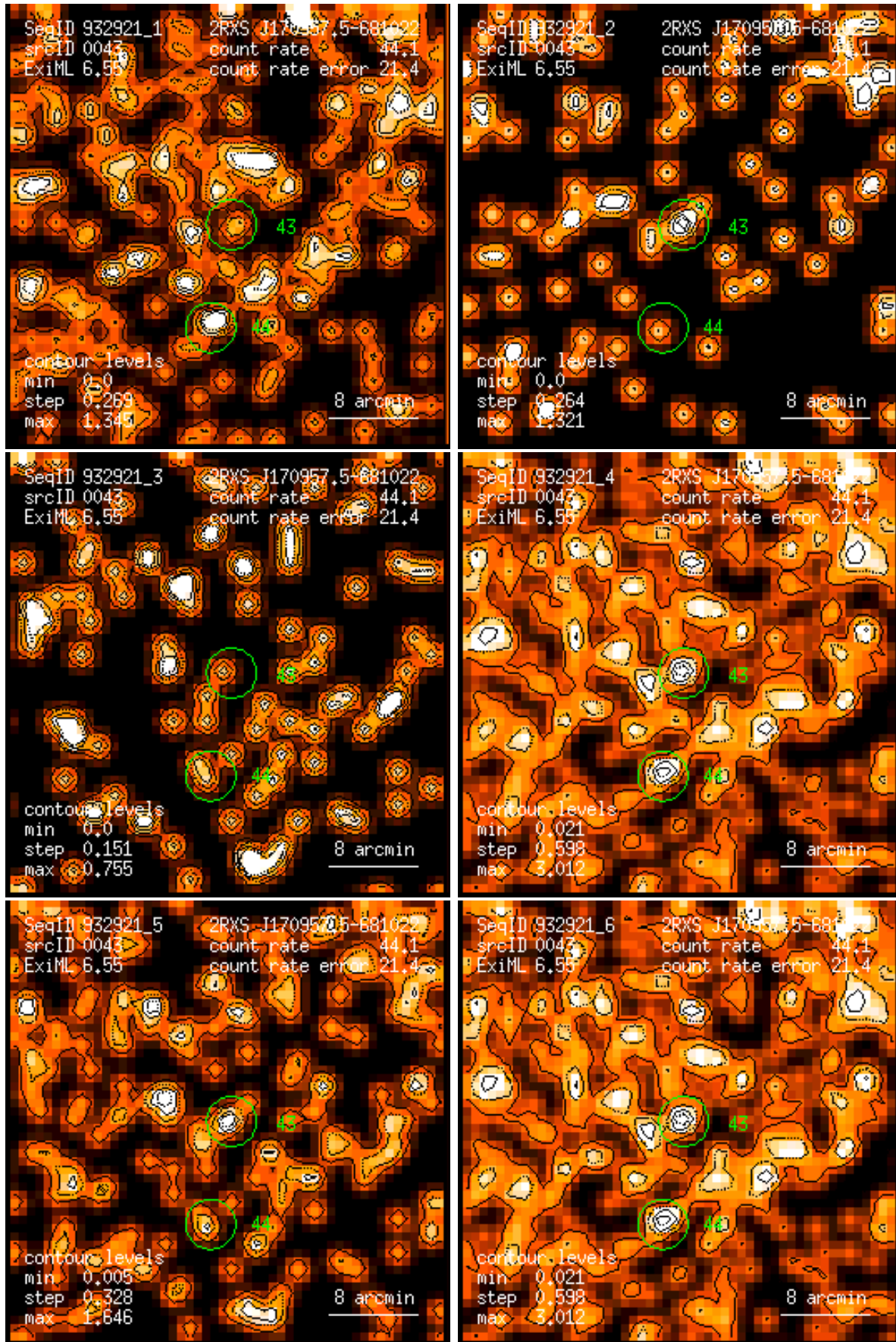
Figure 43: RASS 932921: detection 0043: band rate images, Gaussian filter: (1) PSPC channels 11 – 41, (2) 52 – 90, (3) 91 – 201, (4) 11 – 235, (5) 52 – 201, (6) 11 – 201. Broad band rates in counts/ks. Band rate contour levels in counts/ks/arcmin 2 .
