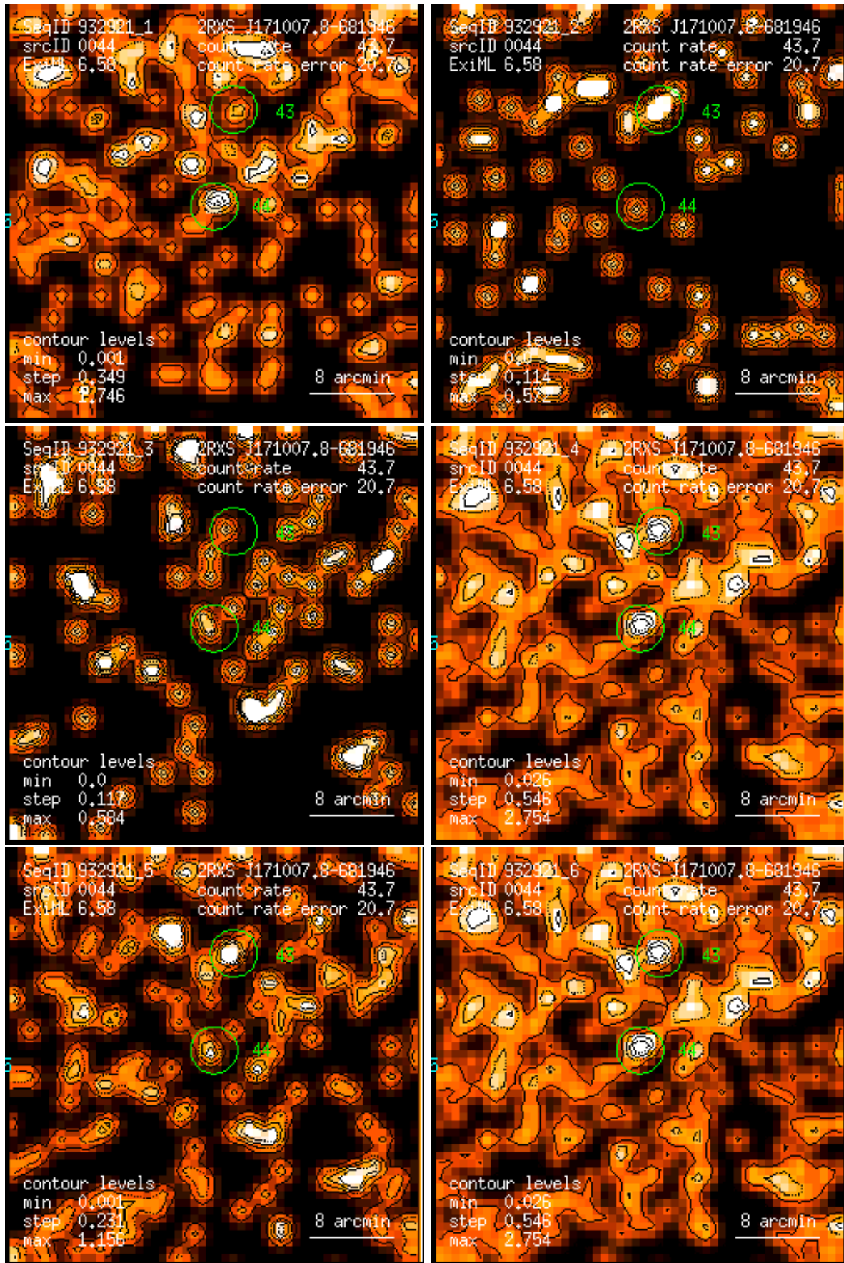
Figure 44: RASS 932921: detection 0044: band rate images, Gaussian filter: (1) PSPC channels 11 – 41, (2) 52 – 90, (3) 91 – 201, (4) 11 – 235, (5) 52 – 201, (6) 11 – 201. Broad band rates in counts/ks. Band rate contour levels in counts/ks/arcmin 2 .
