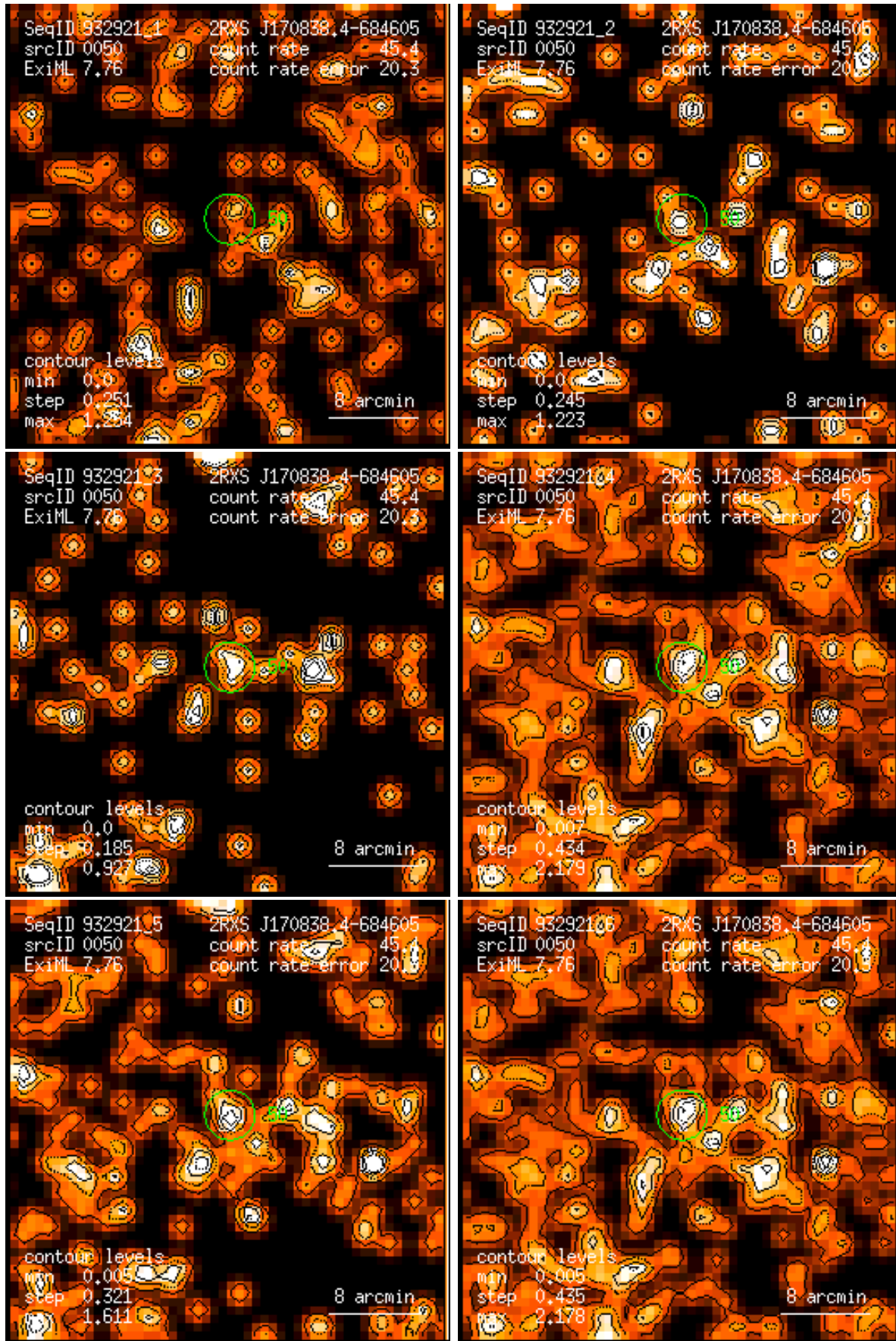
Figure 50: RASS 932921: detection 0050: band rate images, Gaussian filter: (1) PSPC channels 11 – 41, (2) 52 – 90, (3) 91 – 201, (4) 11 – 235, (5) 52 – 201, (6) 11 – 201. Broad band rates in counts/ks. Band rate contour levels in counts/ks/arcmin 2 .
