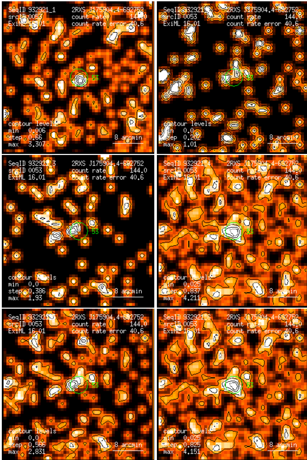
Figure 53: RASS 932921: detection 0053: band rate images, Gaussian filter: (1) PSPC channels 11 – 41, (2) 52 – 90, (3) 91 – 201, (4) 11 – 235, (5) 52 – 201, (6) 11 – 201. Broad band rates in counts/ks. Band rate contour levels in counts/ks/arcmin 2 .
