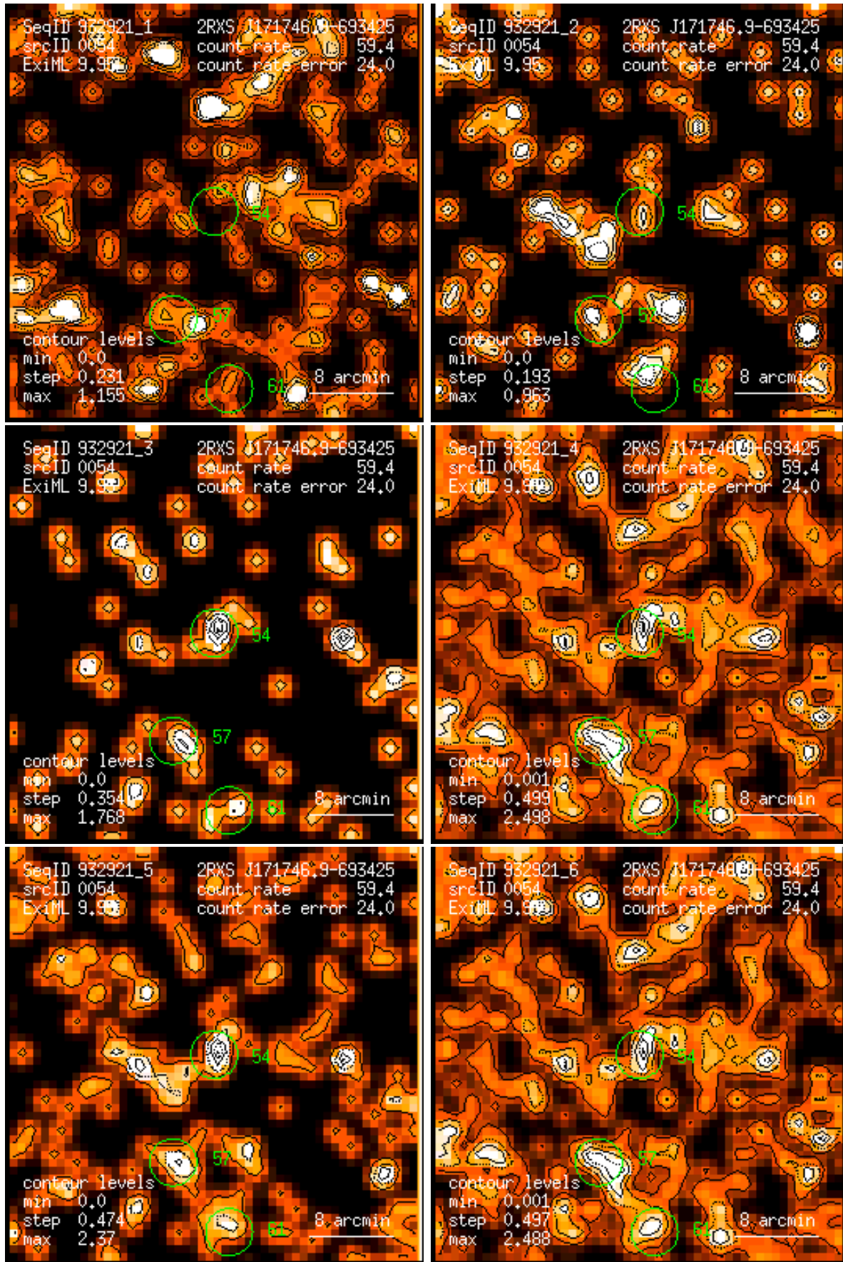
Figure 54: RASS 932921: detection 0054: band rate images, Gaussian filter: (1) PSPC channels 11 – 41, (2) 52 – 90, (3) 91 – 201, (4) 11 – 235, (5) 52 – 201, (6) 11 – 201. Broad band rates in counts/ks. Band rate contour levels in counts/ks/arcmin 2 .
