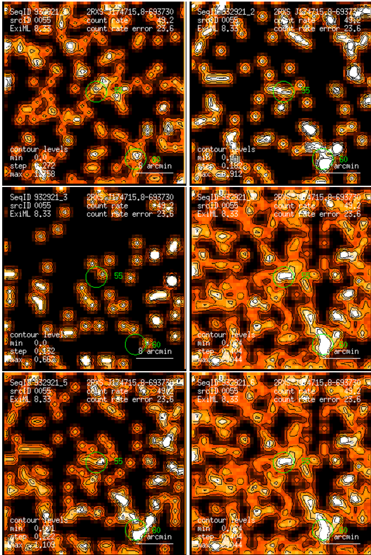
Figure 55: RASS 932921: detection 0055: band rate images, Gaussian filter: (1) PSPC channels 11 – 41, (2) 52 – 90, (3) 91 – 201, (4) 11 – 235, (5) 52 – 201, (6) 11 – 201. Broad band rates in counts/ks. Band rate contour levels in counts/ks/arcmin 2 .
