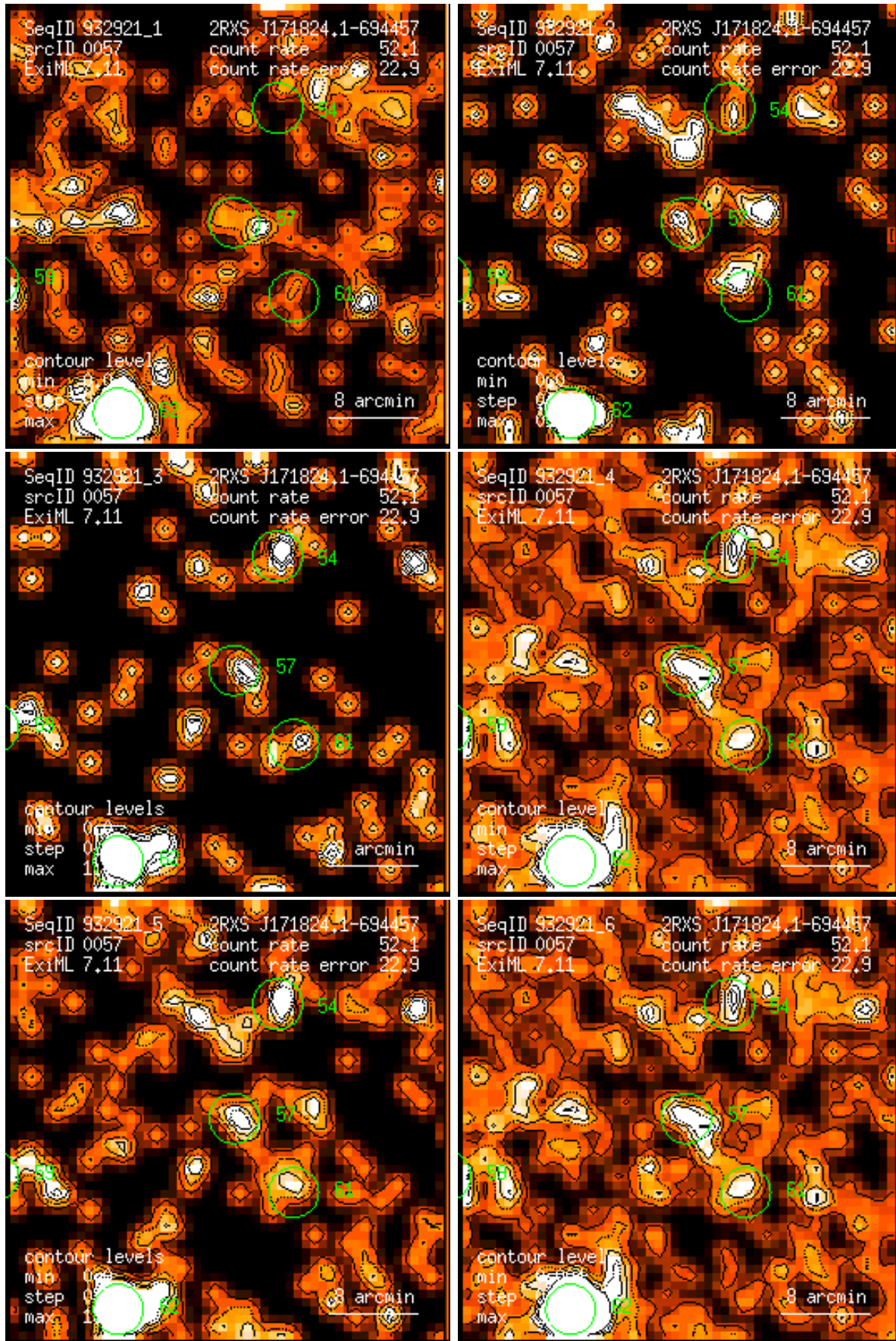
Figure 57: RASS 932921: detection 0057: band rate images, Gaussian filter: (1) PSPC channels 11 – 41, (2) 52 – 90, (3) 91 – 201, (4) 11 – 235, (5) 52 – 201, (6) 11 – 201. Broad band rates in counts/ks. Band rate contour levels in counts/ks/arcmin 2 .
