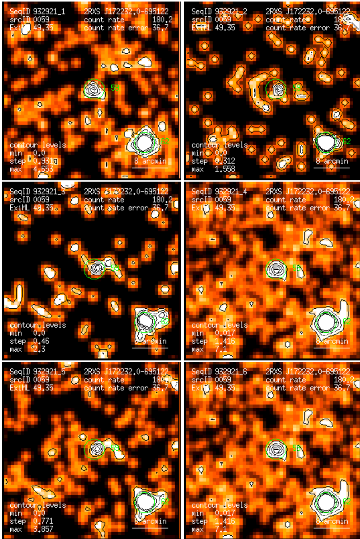
Figure 59: RASS 932921: detection 0059: band rate images, Gaussian filter: (1) PSPC channels 11 – 41, (2) 52 – 90, (3) 91 – 201, (4) 11 – 235, (5) 52 – 201, (6) 11 – 201. Broad band rates in counts/ks. Band rate contour levels in counts/ks/arcmin 2 .
