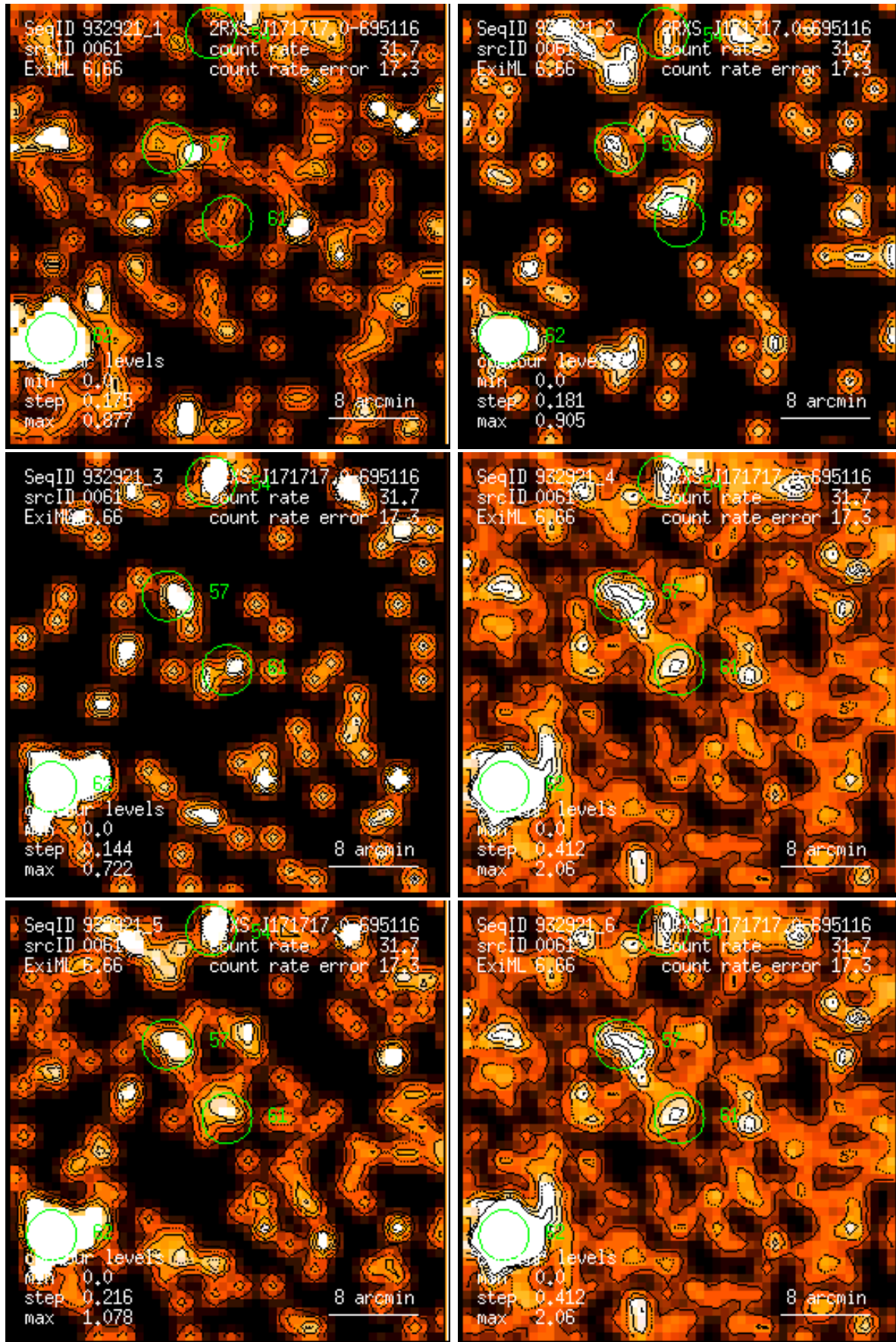
Figure 61: RASS 932921: detection 0061: band rate images, Gaussian filter: (1) PSPC channels 11 – 41, (2) 52 – 90, (3) 91 – 201, (4) 11 – 235, (5) 52 – 201, (6) 11 – 201. Broad band rates in counts/ks. Band rate contour levels in counts/ks/arcmin 2 .
